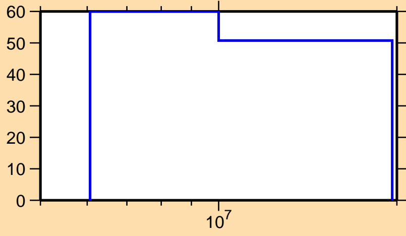
\Delta\sigma/\sigma vs. E for ^{214}\text{Tl}(n,ncont.)
