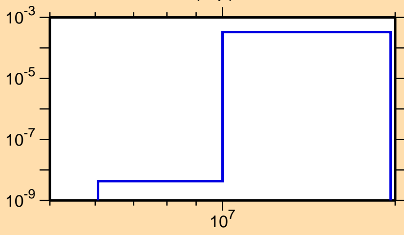
\sigma vs. E for ^{214}\text{Tl}(n,p)
