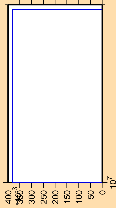
\Delta\sigma/\sigma vs. E for ^{214}\text{Tl}(n,3n\alpha)
