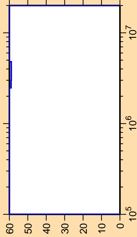
\Delta\sigma/\sigma vs. E for ^{214}\text{Tl}(n,\gamma)
