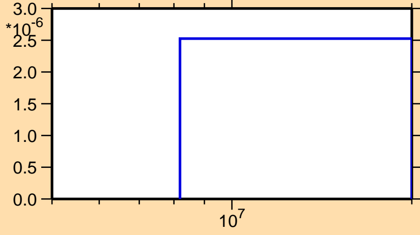
\sigma vs. E for ^{214}\text{Tl}(n,np)
