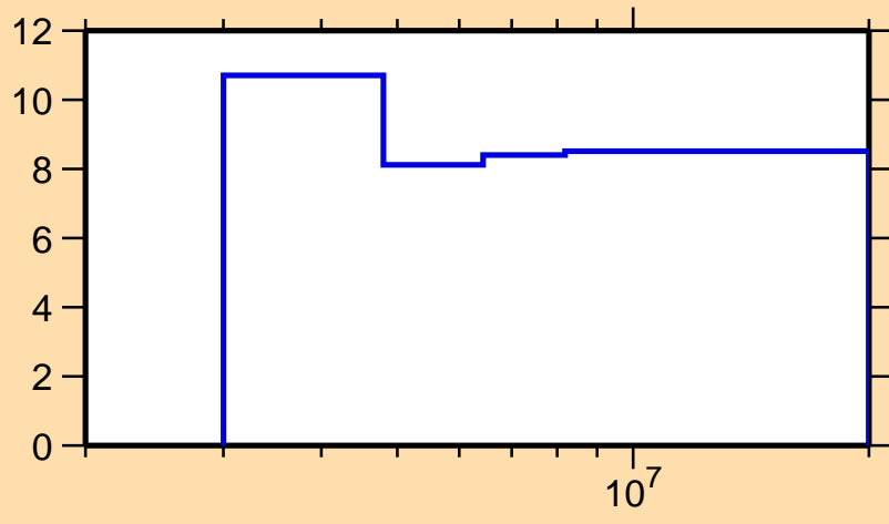
\Delta\sigma/\sigma vs. E for ^{214}\text{Tl}(n,\text{nonel.})
