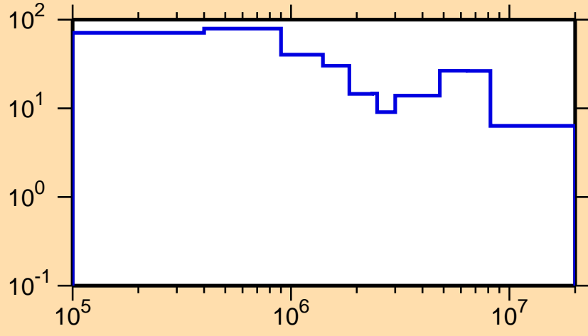
\Delta\sigma/\sigma vs. E for ^{214}\text{Tl}(n, el.)
