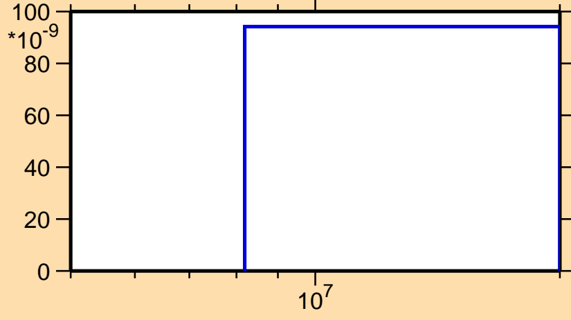
\sigma vs. E for ^{214}\text{Tl}(n,\text{nd})
