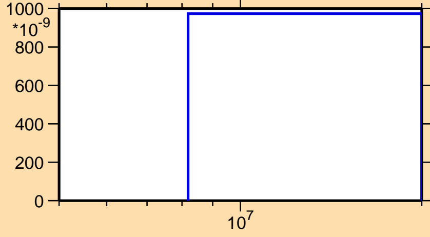
\sigma vs. E for ^{214}\text{Tl}(n,nt)
