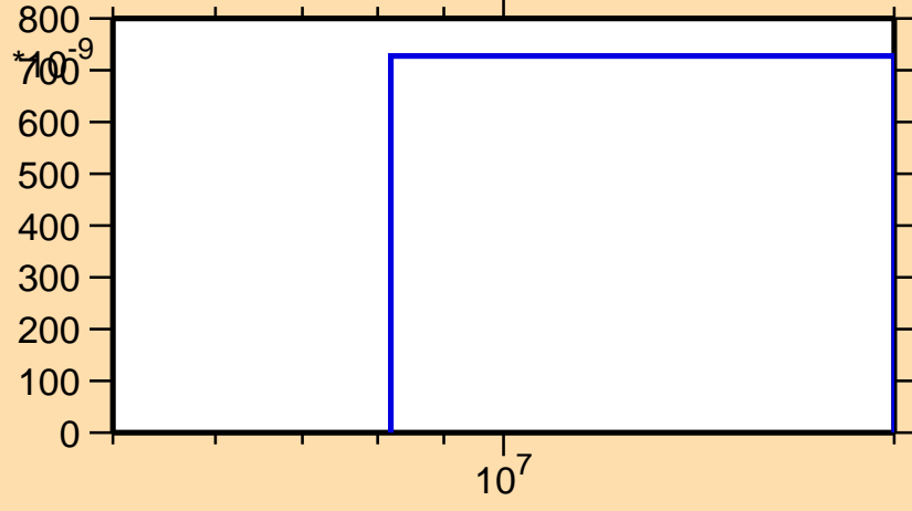
\sigma vs. E for ^{214}\text{Tl}(n,n\alpha)
