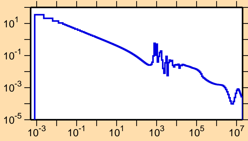
\sigma vs. E for ^{215}\text{Tl}(n,\gamma)
