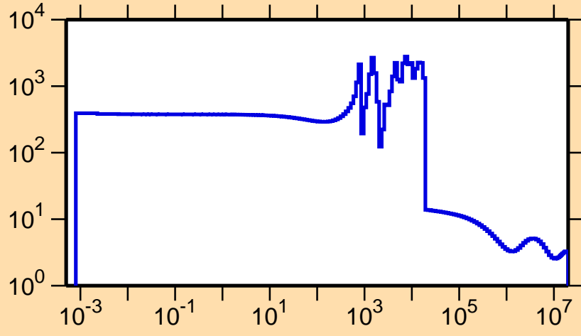
\sigma vs. E for ^{215}\text{Tl}(n,\text{el.})
