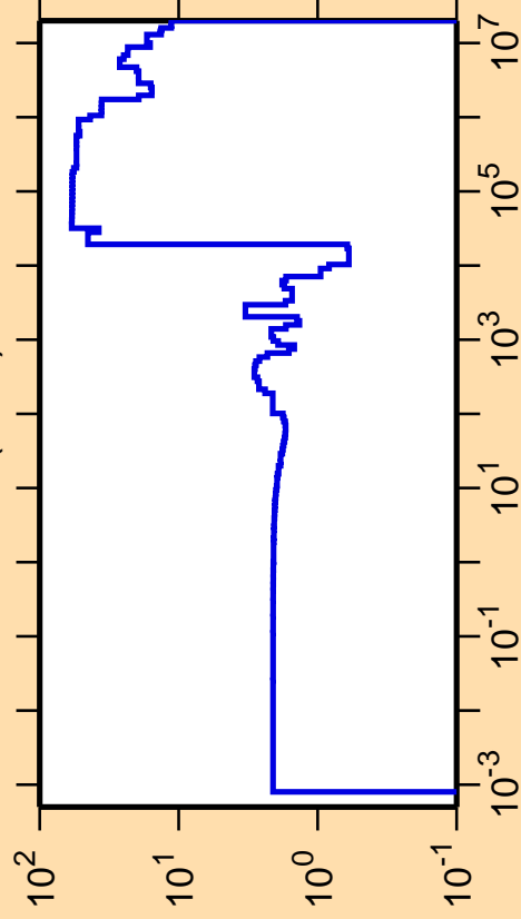
\Delta\sigma/\sigma vs. E for ^{215}\text{Tl}(n,\text{el.})
