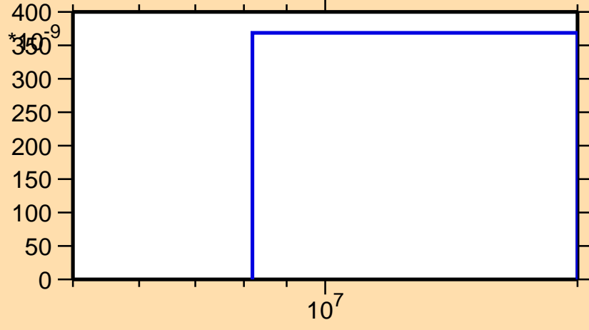
\sigma vs. E for ^{215}\text{Tl}(n,n\alpha)
