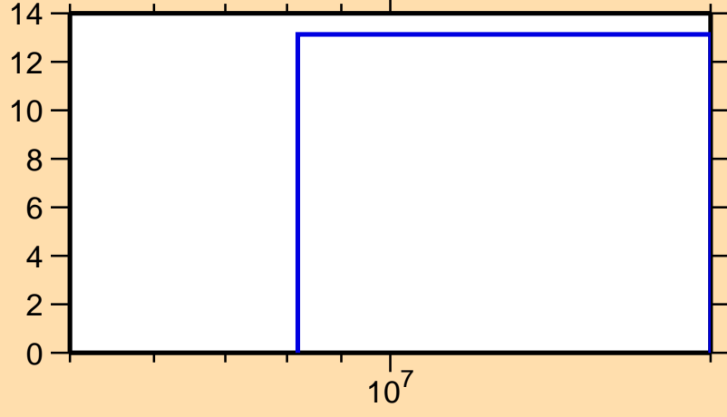
\Delta\sigma/\sigma vs. E for ^{215}\text{Tl}(n,el.)
