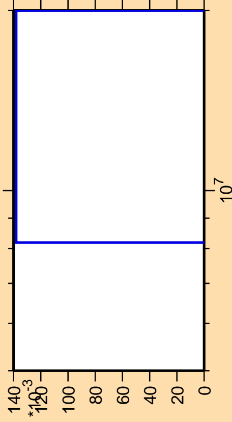
\Delta\sigma/\sigma vs. E for ^{215}\text{Tl}(n,3n\alpha)
