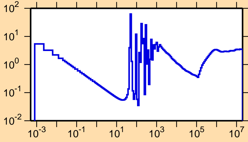
\sigma vs. E for ^{216}\text{Tl}(n,\text{nonel.})
