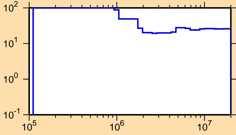
\Delta\sigma/\sigma vs. E for ^{216}\text{Tl}(n, n_{\text{nonel}})
