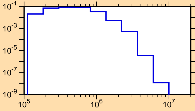
\sigma vs. E for ^{216}\text{Tl}(n,n_1)
