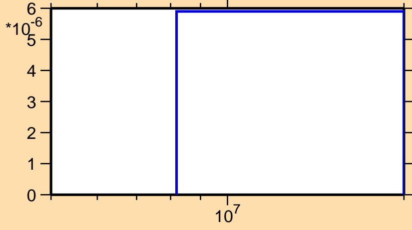
\sigma vs. E for ^{216}\text{Tl}(n,n\alpha)
