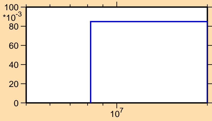
\sigma vs. E for ^{216}\text{Tl}(n,nt)
