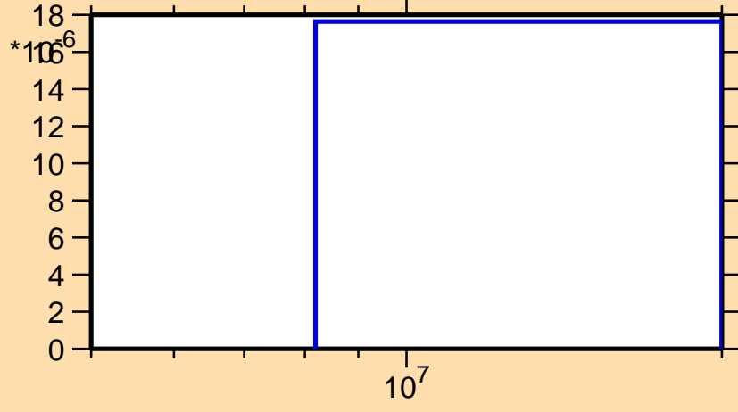
\sigma vs. E for ^{216}\text{Tl}(n,np)
