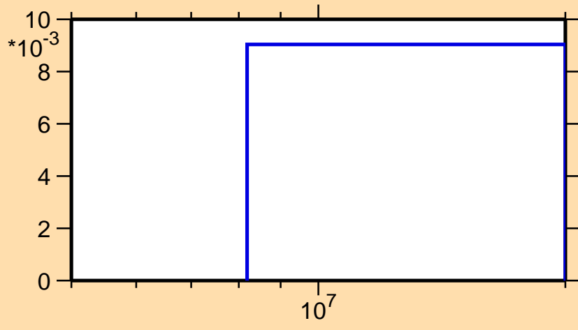
\sigma vs. E for ^{216}\text{Tl}(n,nd)
