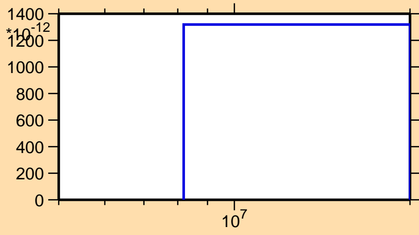
\sigma vs. E for ^{216}\text{Tl}(n,2n\alpha)
