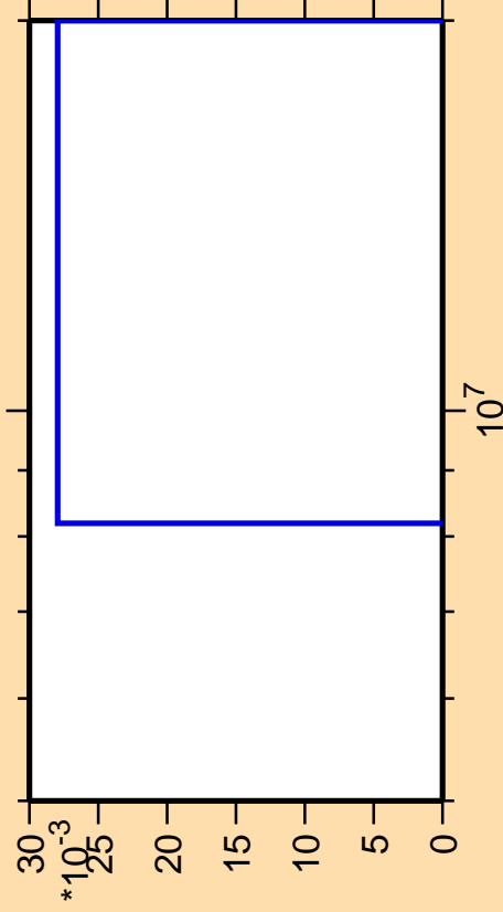
\Delta\sigma/\sigma vs. E for ^{216}\text{Tl}(n,3n\alpha)
