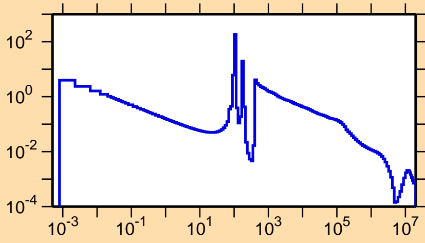
\sigma vs. E for ^{217}\text{Tl}(n,\gamma)
