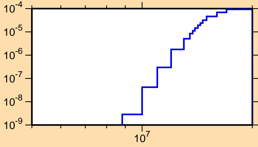
\sigma vs. E for ^{217}\text{Tl}(n,\alpha)
