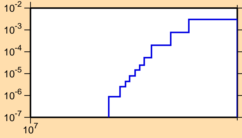
\sigma vs. E for ^{217}\text{Tl}(n,2n\alpha)
