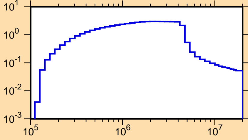
\sigma vs. E for ^{217}\text{Tl}(n,n\text{cont.})
