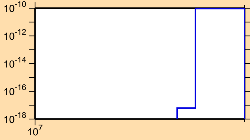
\sigma vs. E for ^{217}\text{Tl} (mt 11)
