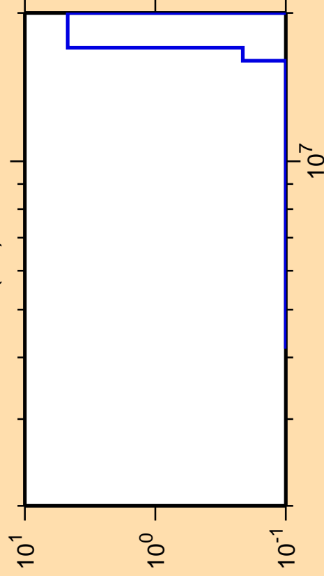
\Delta\sigma/\sigma vs. E for ^{217}\text{Tl}(n,f)
