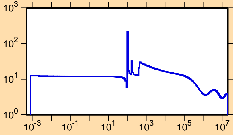
\sigma vs. E for ^{217}\text{Tl}(n,\text{el.})
