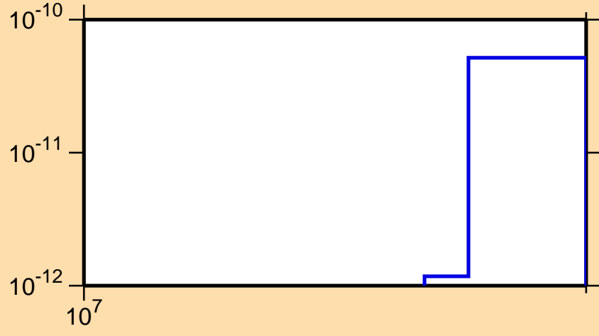
\sigma vs. E for ^{217}\text{Tl}(n,3n\alpha)
