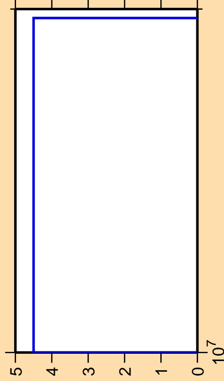
\Delta\sigma/\sigma vs. E for ^{217}\text{Tl}(n,3n\alpha)
