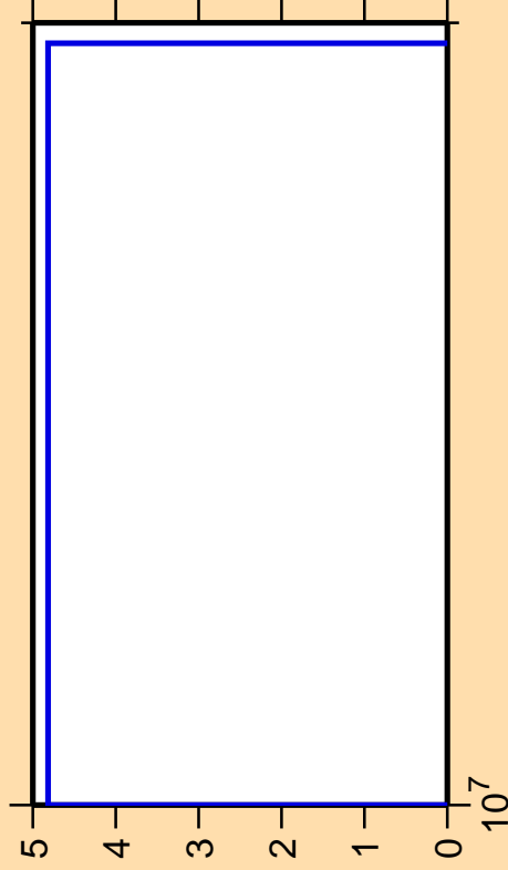
\Delta\sigma/\sigma vs. E for ^{217}\text{Tl} (mt 11)
