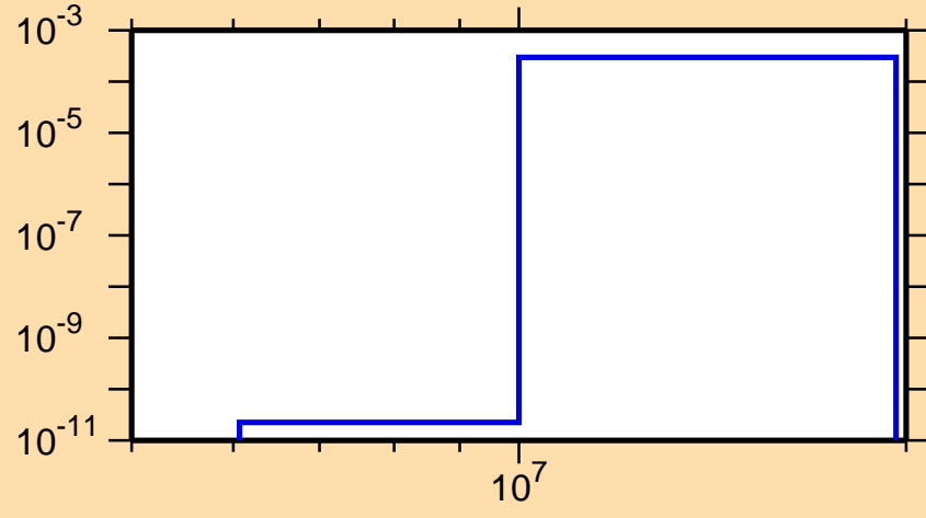
\sigma vs. E for ^{217}\text{Tl}(n,p)
