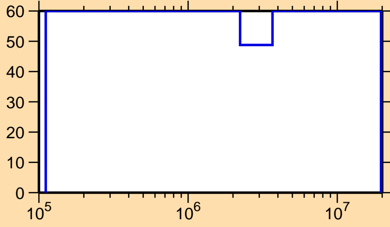
\Delta\sigma/\sigma vs. E for ^{217}\text{Tl}(n, tot.)
