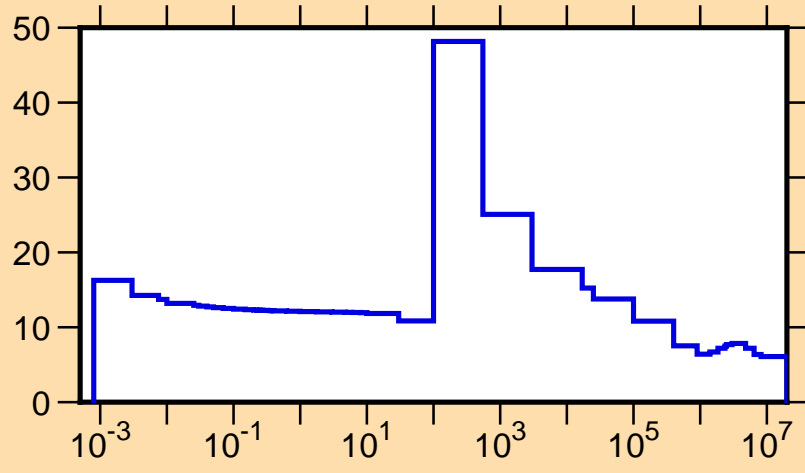
\sigma vs. E for ^{217}\text{Tl}(n,\text{tot.})
