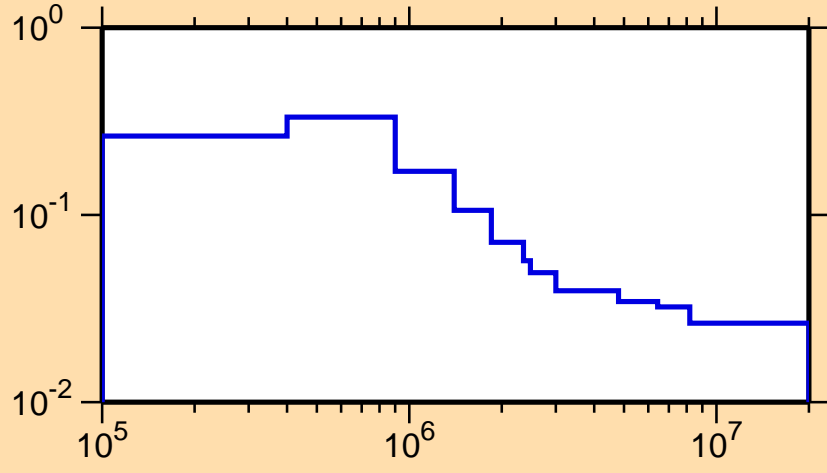
\sigma vs. E for ^{217}\text{Tl}(n,n_1)
