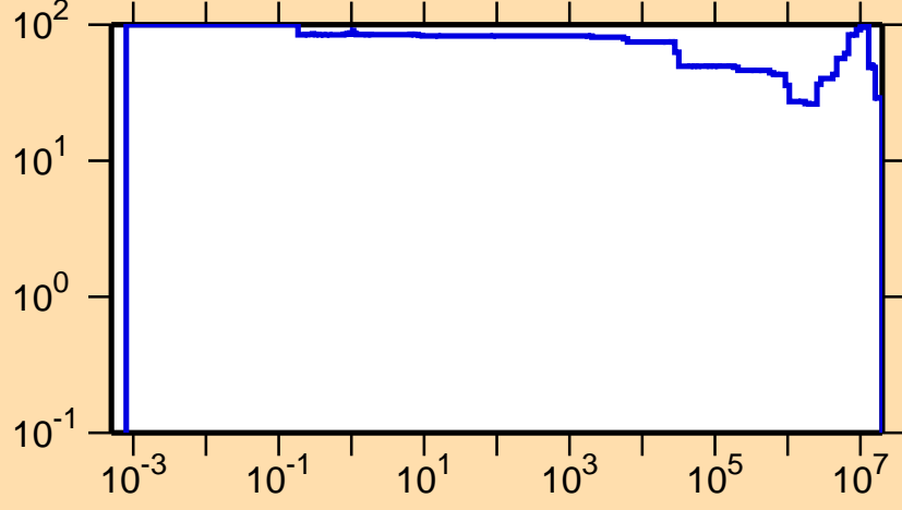
\Delta\sigma/\sigma vs. E for ^{150}\text{Tm}(n,p)
