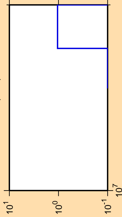
\Delta\sigma/\sigma vs. E for ^{150}\text{Tm}(n,nt)
