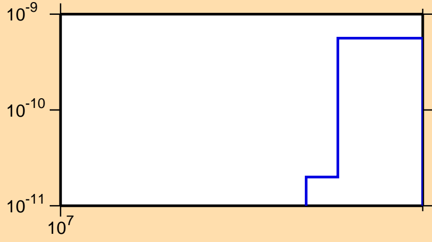
\sigma vs. E for ^{150}\text{Tm}(n,2n\alpha)
