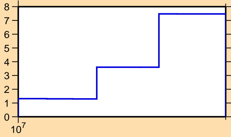
\Delta\sigma/\sigma vs. E for ^{150}\text{Tm}(n,\text{tot.})
