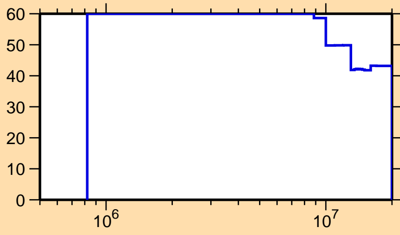
\Delta\sigma/\sigma vs. E for ^{150}\text{Tm}(n,n\text{cont.})
