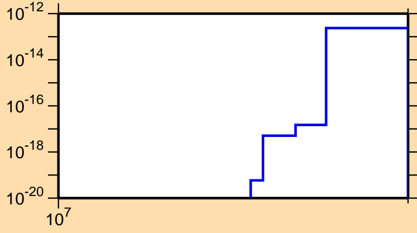
\sigma vs. E for ^{150}\text{Tm}(n,nt)
