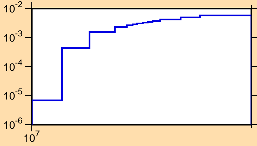
\sigma vs. E for ^{150}\text{Tm}(n,2n)
