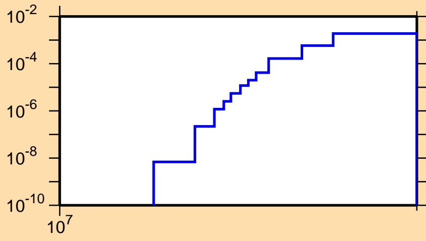
\sigma vs. E for ^{150}\text{Tm}(n,2np)
