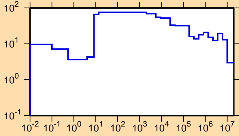
\Delta\sigma/\sigma vs. E for ^{150}\text{Tm}(n,tot.)
