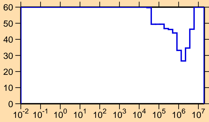
\Delta\sigma/\sigma vs. E for ^{150}\text{Tm}(n,p)
