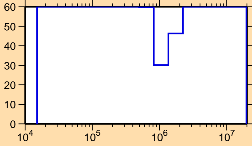
\Delta\sigma/\sigma vs. E for ^{150}\text{Tm}(n,n_1)
