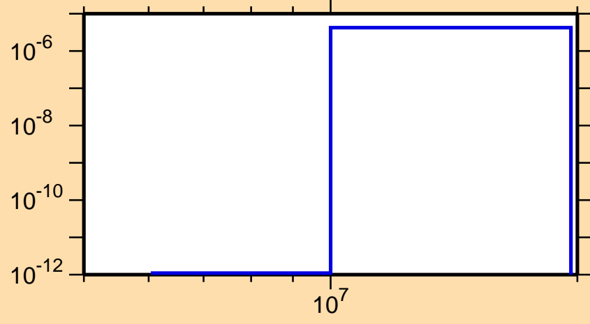
\sigma vs. E for ^{150}\text{Tm} (mt 45)
