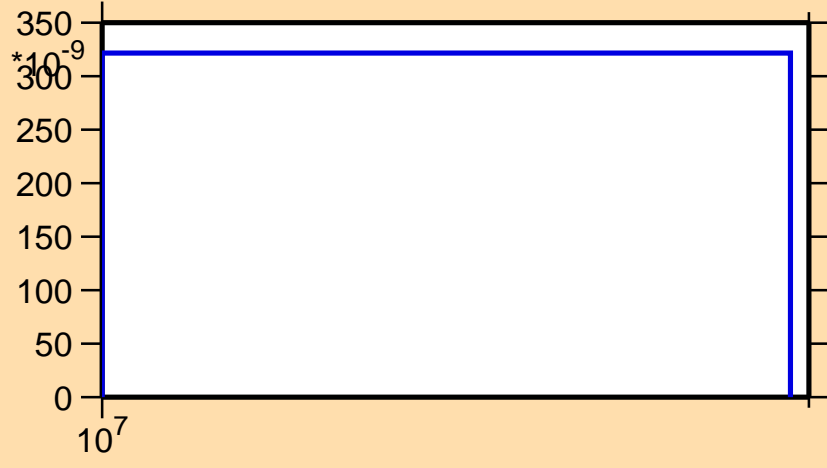
\sigma vs. E for ^{150}\text{Tm}(n,nd)
