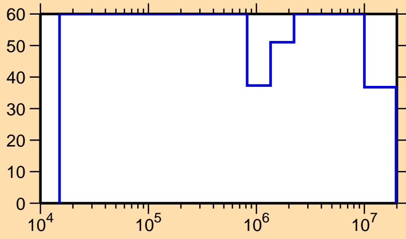
\Delta\sigma/\sigma vs. E for ^{150}\text{Tm}(n,\text{inel.})
