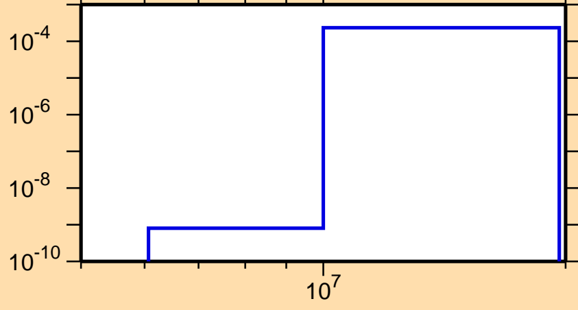
\sigma vs. E for ^{150}\text{Tm}(n,\text{pd})
