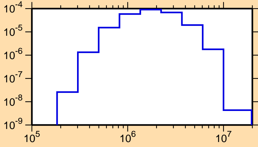
\sigma vs. E for ^{150}\text{Tm}(n,n_3)
