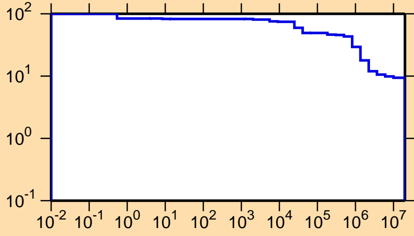
\Delta\sigma/\sigma vs. E for ^{150}\text{Tm}(n,\text{nonel.})
