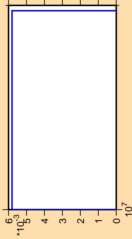
\Delta\sigma/\sigma vs. E for ^{150}\text{Tm}(n,nt)
