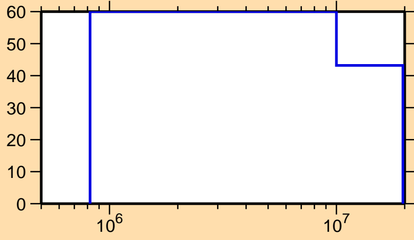
\Delta\sigma/\sigma vs. E for ^{150}\text{Tm}(n,n\text{cont.})
