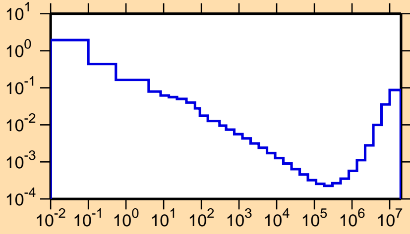
\sigma vs. E for ^{150}\text{Tm}(n,\alpha)
