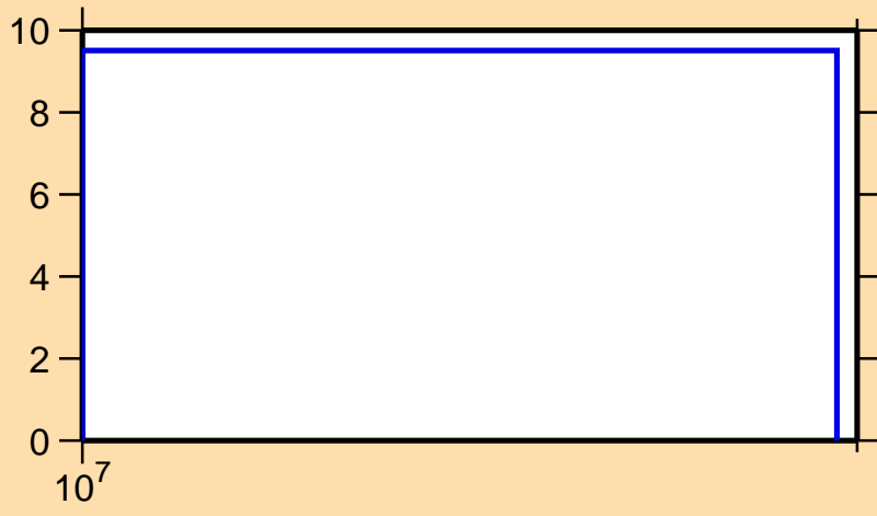
\Delta\sigma/\sigma vs. E for ^{150}\text{Tm}(n,\text{el.})
