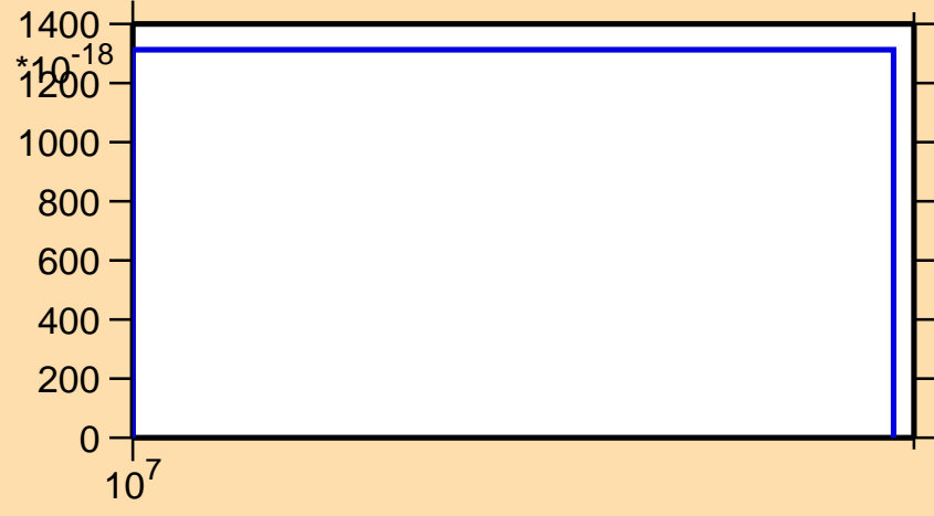
\sigma vs. E for ^{150}\text{Tm}(n,nt)
