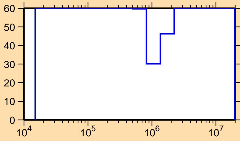
\Delta\sigma/\sigma vs. E for ^{150}\text{Tm}(n,n_1)
