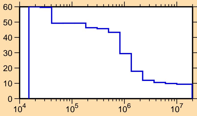
\Delta\sigma/\sigma vs. E for ^{150}\text{Tm}(n,\text{nonel.})
