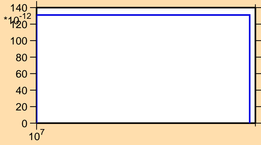
\sigma vs. E for ^{150}\text{Tm} (mt 34)
