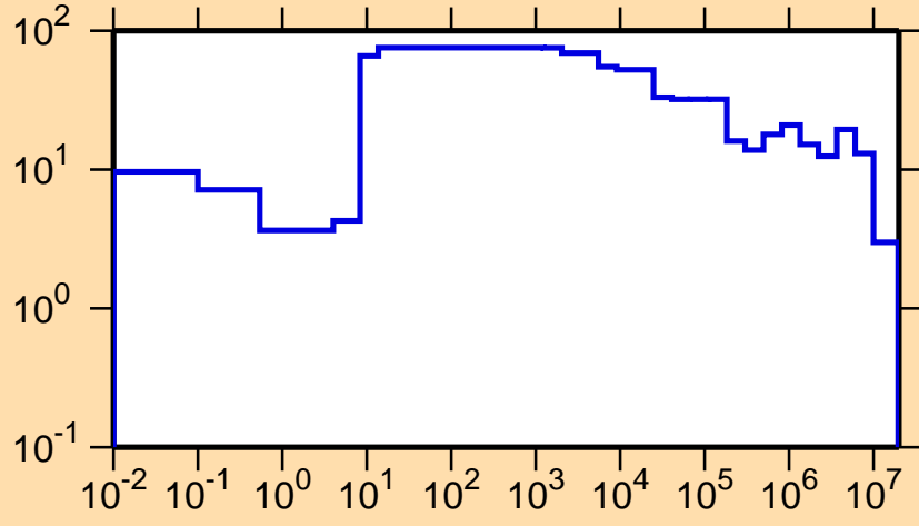
\Delta\sigma/\sigma vs. E for ^{150}\text{Tm}(n,\text{tot.})
