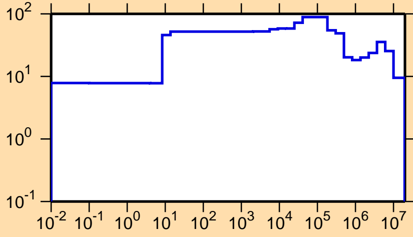
\Delta\sigma/\sigma vs. E for ^{150}\text{Tm}(n,\text{el.})
