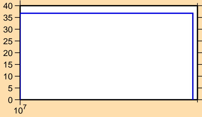
\Delta\sigma/\sigma vs. E for ^{150}\text{Tm}(n,\text{inel.})
