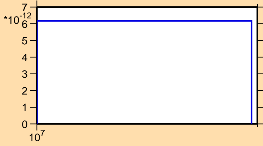
\sigma vs. E for ^{150}\text{Tm}(n,2n\alpha)
