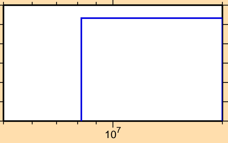
\sigma vs. E for ^{150}\text{Tm}(\text{mt117})
