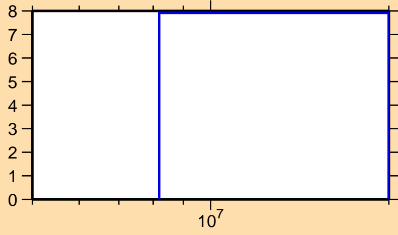
\Delta\sigma/\sigma vs. E for ^{150}\text{Tm}(n,\text{el.})
