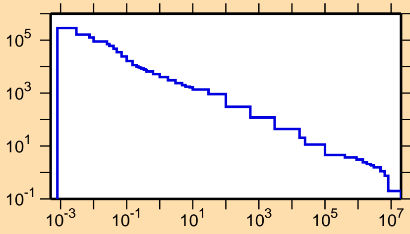
\sigma vs. E for ^{150}\text{Tm}(n,p)
