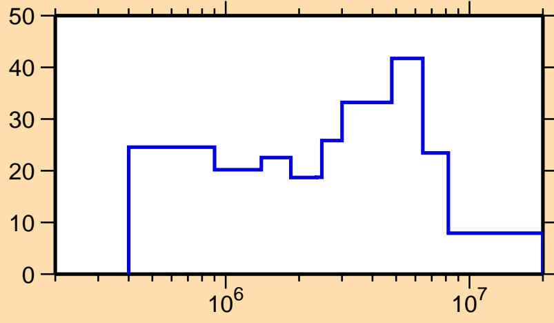
\Delta\sigma/\sigma vs. E for ^{150}\text{Tm}(n, el.)
