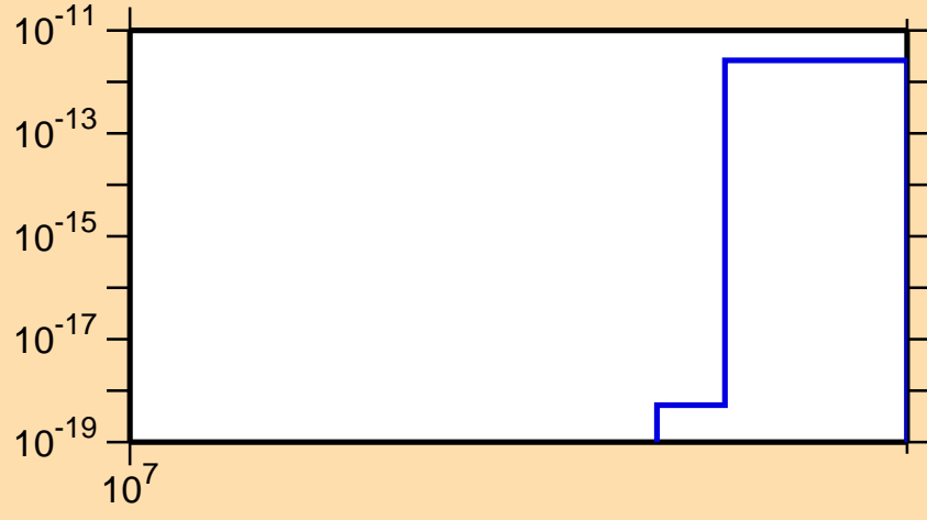
\sigma vs. E for ^{151}\text{Tm}(n,nt)
