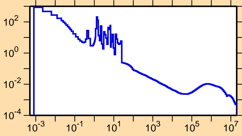
\sigma vs. E for ^{151}\text{Tm}(n,\gamma)
