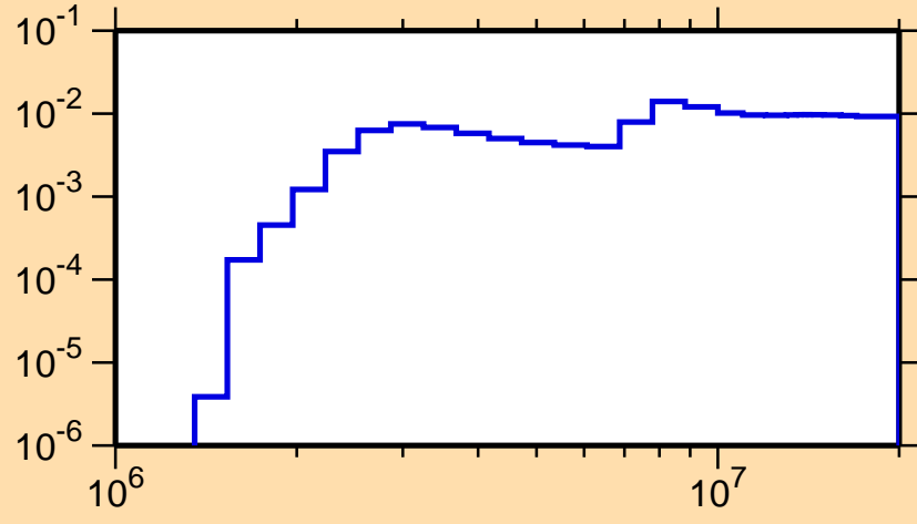
\sigma vs. E for ^{151}\text{Tm}(n,n\text{cont.})
