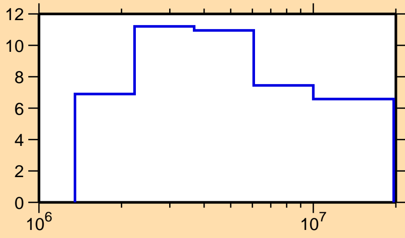
\Delta\sigma/\sigma vs. E for ^{151}\text{Tm}(n, nonel.)
