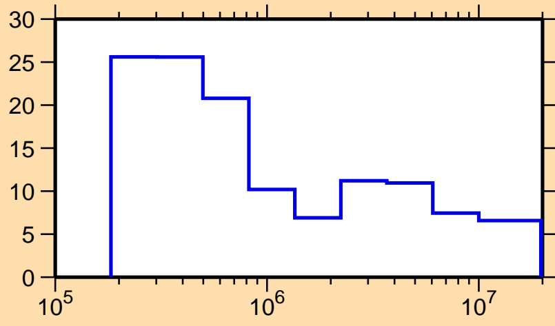
\Delta\sigma/\sigma vs. E for ^{151}\text{Tm}(n,\text{nonel.})
