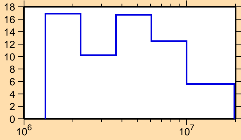
\Delta\sigma/\sigma vs. E for ^{151}\text{Tm}(n, el.)
