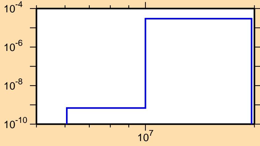
\sigma vs. E for ^{151}\text{Tm} (mt 45)
