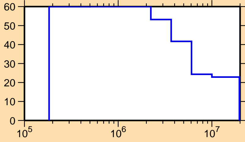
\Delta\sigma/\sigma vs. E for ^{151}\text{Tm}(n,n_1)
