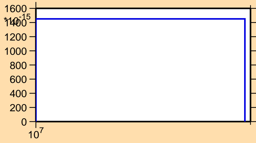
\sigma vs. E for ^{151}\text{Tm} (mt 34)
