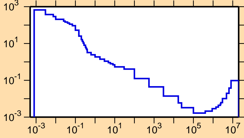
\sigma vs. E for ^{151}\text{Tm}(n,\alpha)
