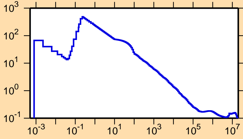
\sigma vs. E for ^{152}\text{Tm}(n,\alpha)
