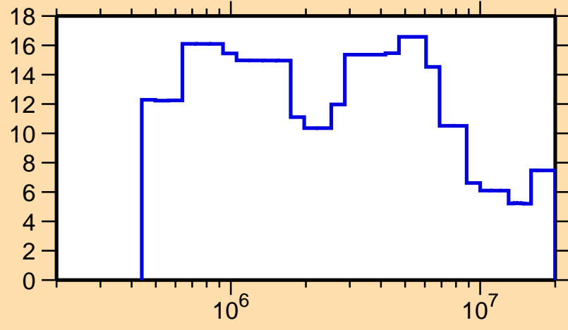
\Delta\sigma/\sigma vs. E for ^{152}\text{Tm}(n, tot.)
