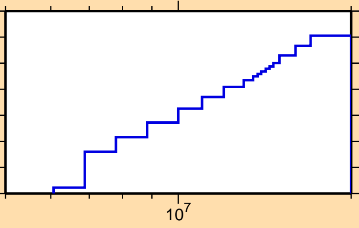
\sigma vs. E for ^{152}\text{Tm}(\text{mt117})
