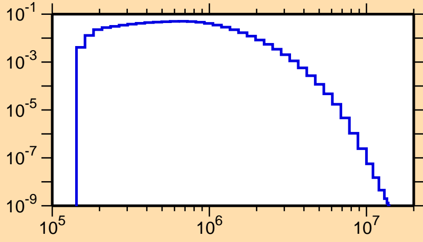
\sigma vs. E for ^{152}\text{Tm}(n,n_1)
