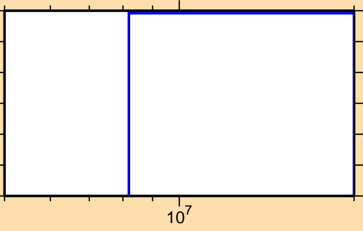
\sigma vs. E for ^{152}\text{Tm}(n,nt)
