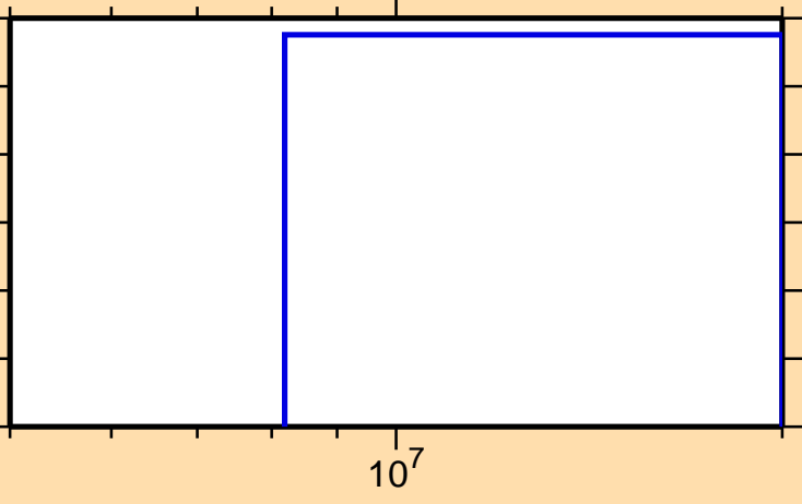
\sigma vs. E for ^{152}\text{Tm}(n,2n\alpha)
