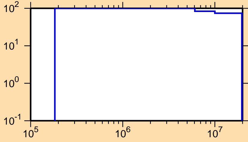
\Delta\sigma/\sigma vs. E for ^{152}\text{Tm}(n,ncont.)
