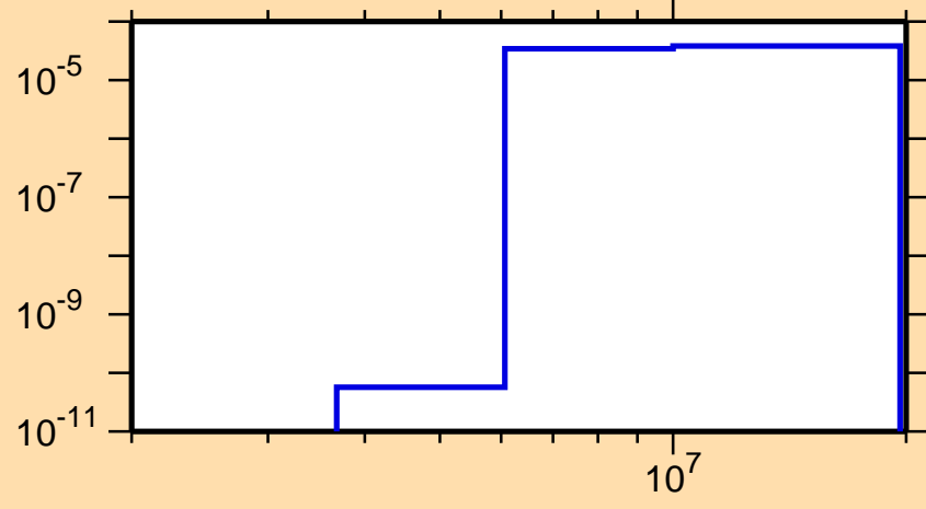
\sigma vs. E for ^{152}\text{Tm} (mt 45)
