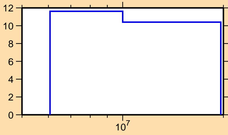
\Delta\sigma/\sigma vs. E for ^{152}\text{Tm}(n,\text{nonel.})
