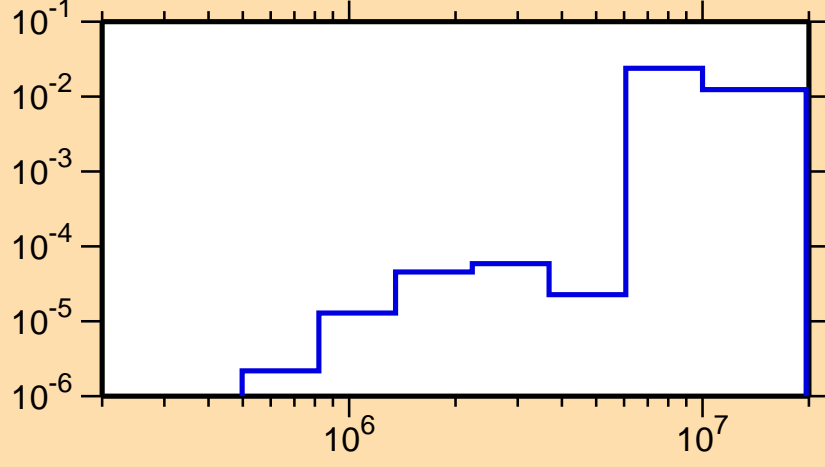
\sigma vs. E for ^{152}\text{Tm}(n,\text{inel.})
