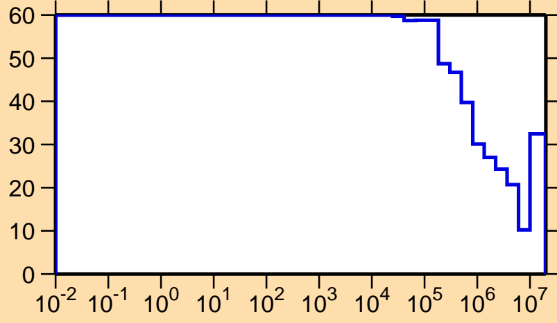
\Delta\sigma/\sigma vs. E for ^{152}\text{Tm}(n,p)
