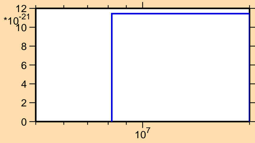
\sigma vs. E for ^{152}\text{Tm} (mt 11)
