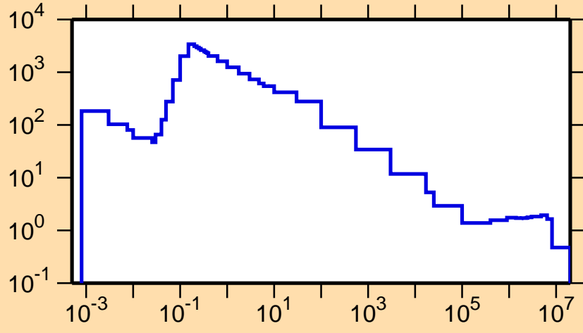
\sigma vs. E for ^{152}\text{Tm}(n,p)
