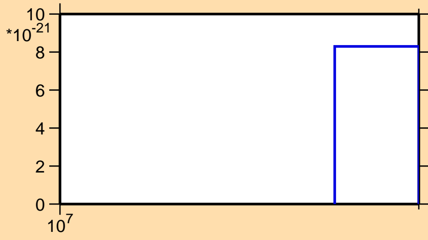
\sigma vs. E for ^{153}\text{Tm} (mt 42)
