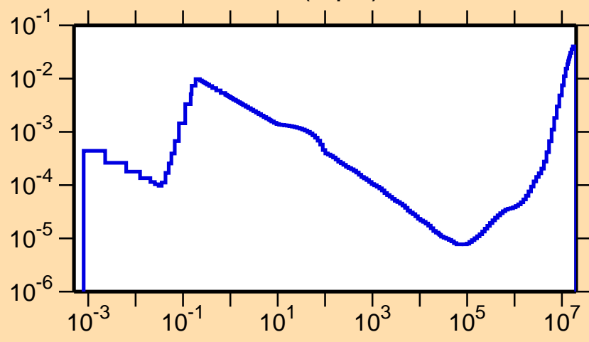
\sigma vs. E for ^{153}\text{Tm}(n,p\alpha)
