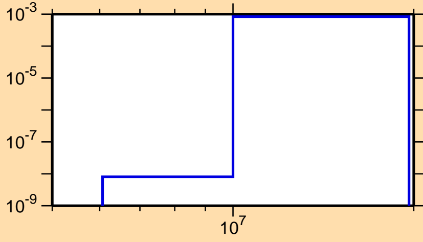
\sigma vs. E for ^{153}\text{Tm}(n,t)
