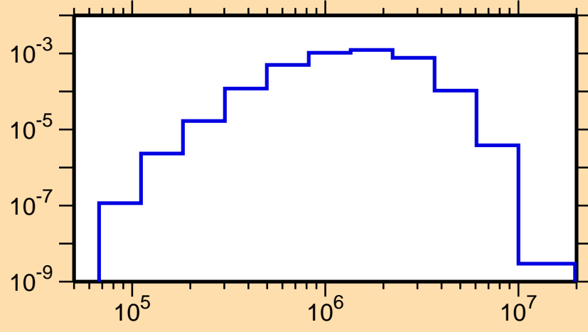
\sigma vs. E for ^{153}\text{Tm}(n,n_1)
