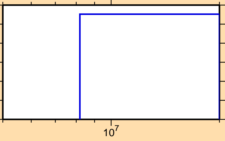
\sigma vs. E for ^{153}\text{Tm}(n,3n)
