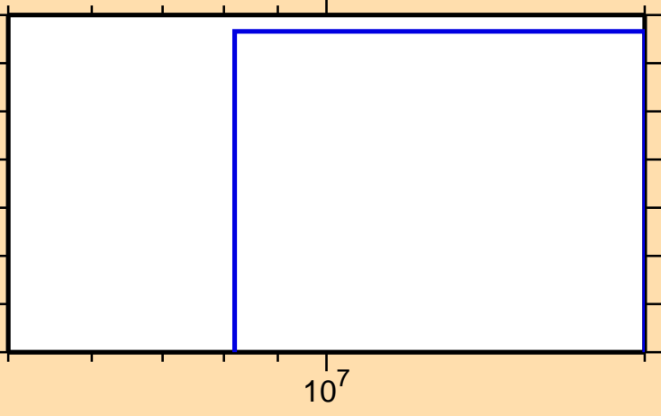
\sigma vs. E for ^{153}\text{Tm}(n,2n)
