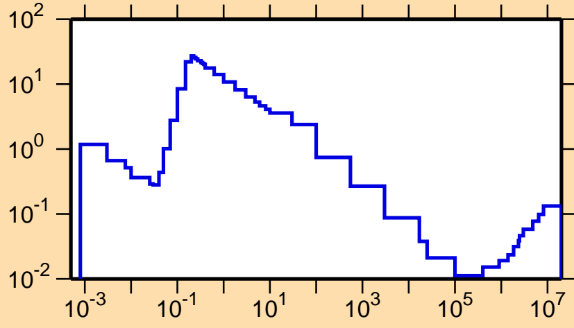
\sigma vs. E for ^{153}\text{Tm}(n,\alpha)
