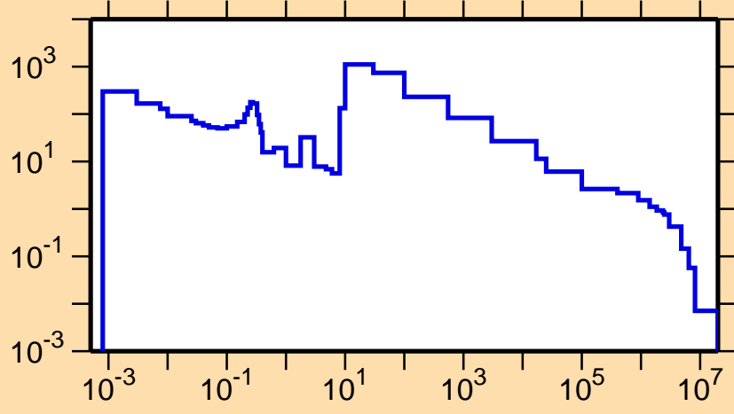
\sigma vs. E for ^{153}\text{Tm}(n,\gamma)
