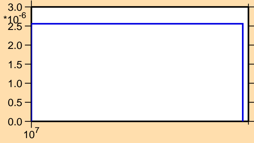
\sigma vs. E for ^{153}\text{Tm}(n,\text{nd})
