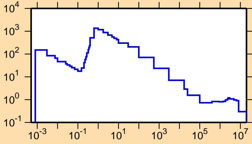
\sigma vs. E for ^{153}\text{Tm}(n,p)
