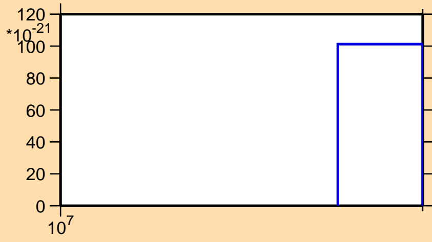
\sigma vs. E for ^{154}\text{Tm} (mt 42)
