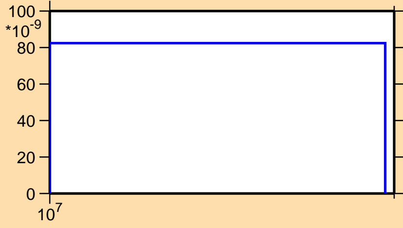
\sigma vs. E for ^{154}\text{Tm}(n,pt)
