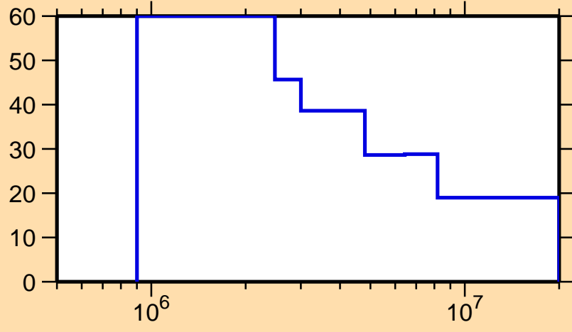
\Delta\sigma/\sigma vs. E for ^{154}\text{Tm}(n,ncont.)
