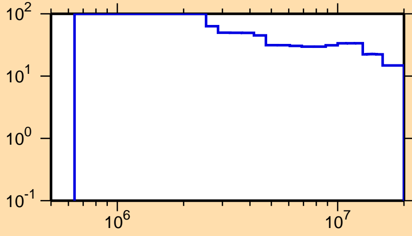
\Delta\sigma/\sigma vs. E for ^{154}\text{Tm}(n,n\text{cont.})
