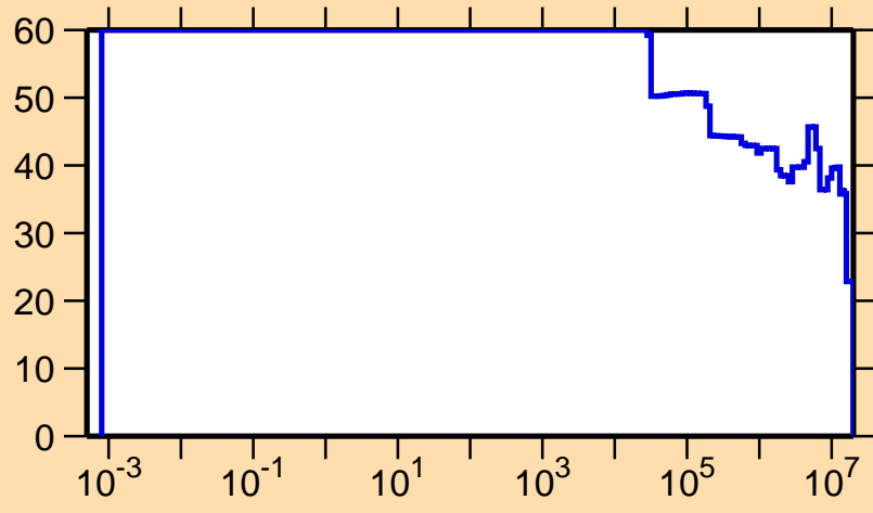
\Delta\sigma/\sigma vs. E for ^{154}\text{Tm}(n,p)
