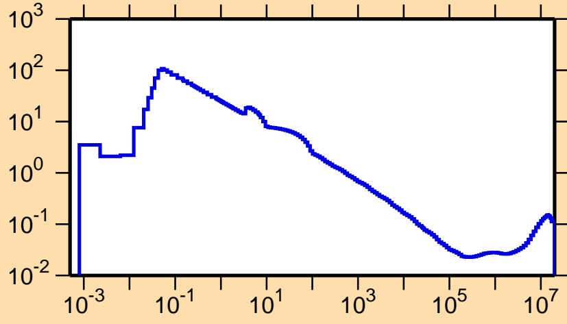
\sigma vs. E for ^{154}\text{Tm}(n,\alpha)
