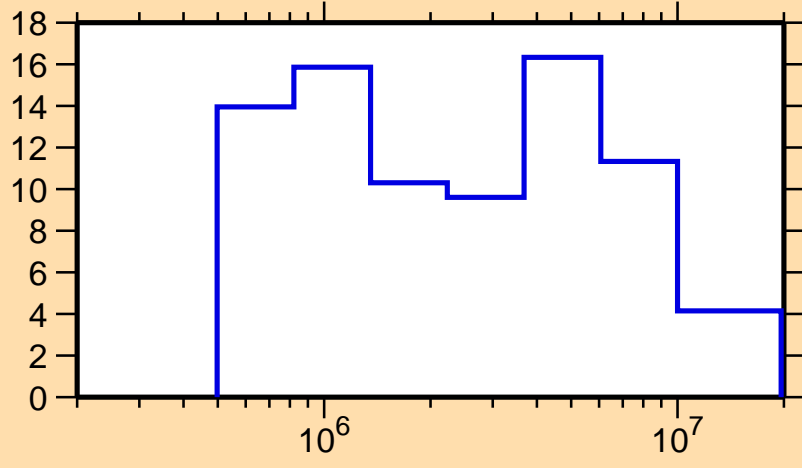
\Delta\sigma/\sigma vs. E for ^{154}\text{Tm}(n, tot.)
