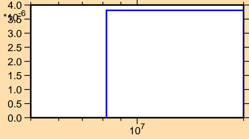
\sigma vs. E for ^{154}\text{Tm}(n,nd)
