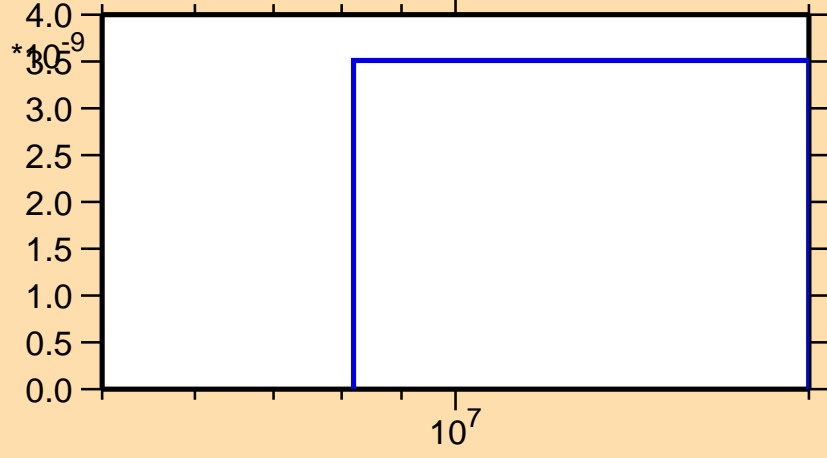
\sigma vs. E for ^{154}\text{Tm}(n,nt)
