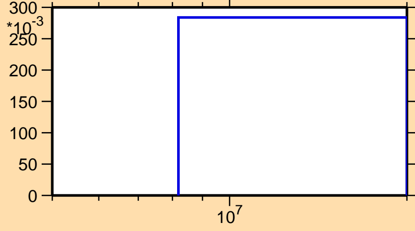
\sigma vs. E for ^{154}\text{Tm}(n,2n)
