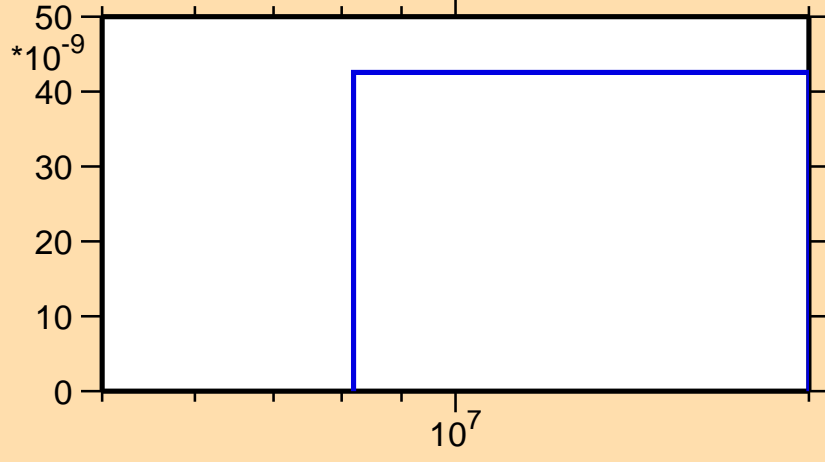
\sigma vs. E for ^{154}\text{Tm}(n,\text{pt})
