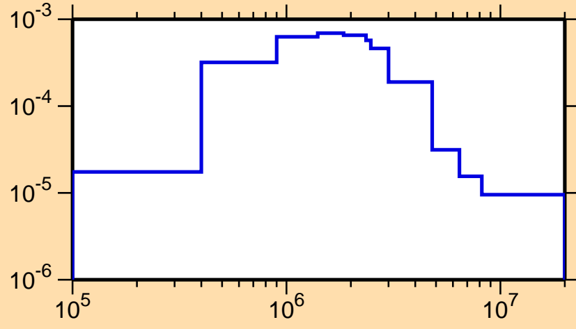
\sigma vs. E for ^{155}\text{Tm}(n,n_1)
