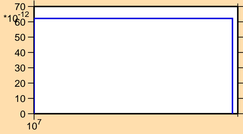
\sigma vs. E for ^{155}\text{Tm}(n,\text{pt})
