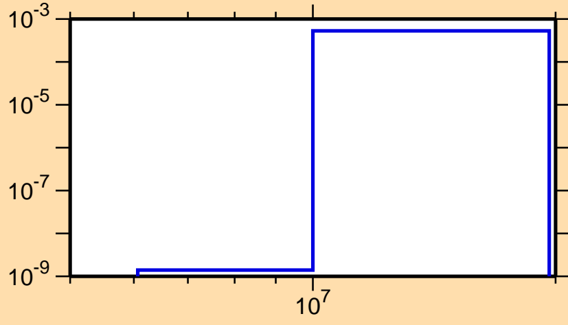
\sigma vs. E for ^{155}\text{Tm}(n,t)
