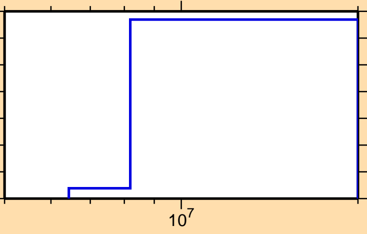
\sigma vs. E for ^{155}\text{Tm}(n,\text{He}3)
