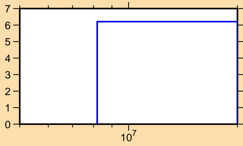
\Delta\sigma/\sigma vs. E for ^{155}\text{Tm}(n,\text{nonel.})
