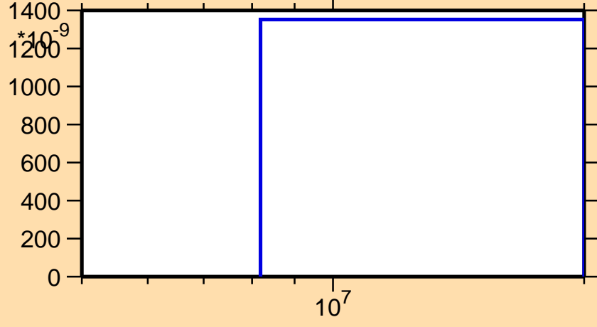
\sigma vs. E for ^{155}\text{Tm}(n,2n\alpha)
