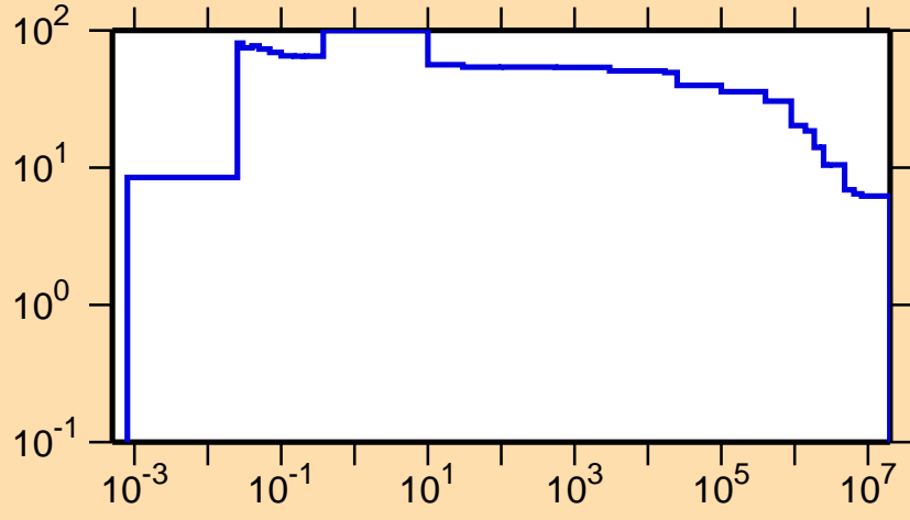
\Delta\sigma/\sigma vs. E for ^{155}\text{Tm}(n,\text{nonel.})
