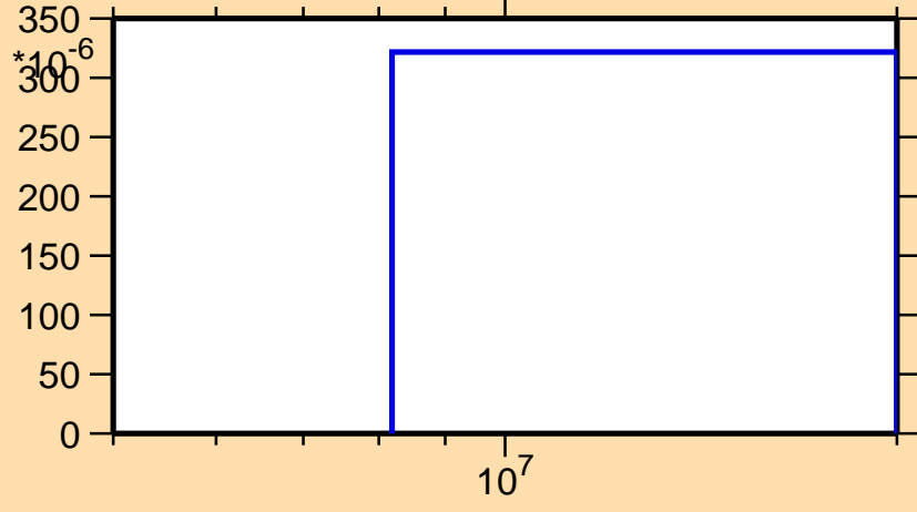
\sigma vs. E for ^{155}\text{Tm}(n,2np)
