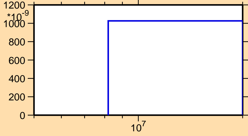
\sigma vs. E for ^{155}\text{Tm}(n,\text{nd})
