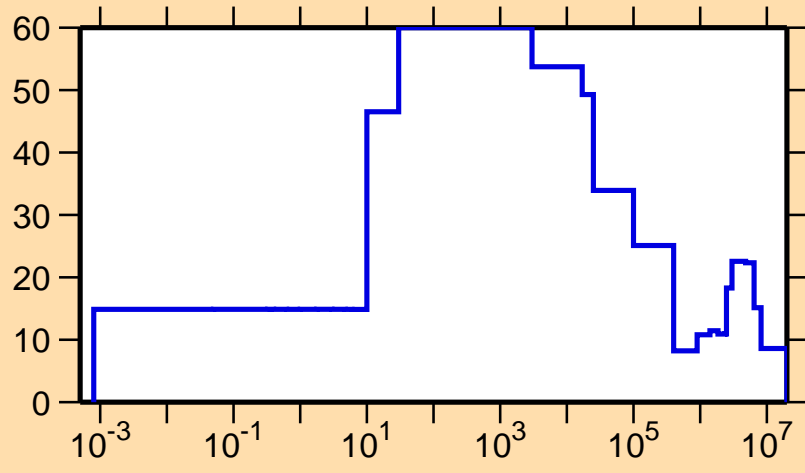
\Delta\sigma/\sigma vs. E for ^{155}\text{Tm}(n,\text{el.})
