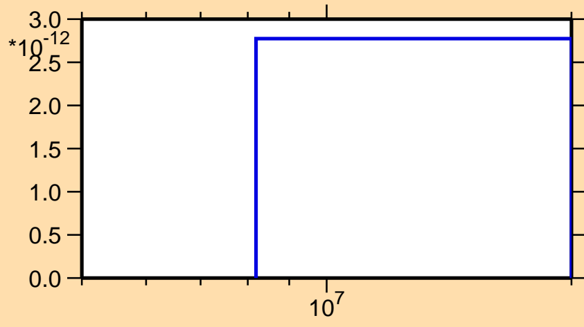
\sigma vs. E for ^{155}\text{Tm} (mt 34)
