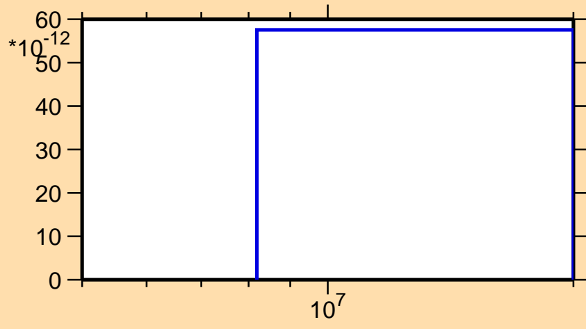
\sigma vs. E for ^{155}\text{Tm}(n,\text{pt})
