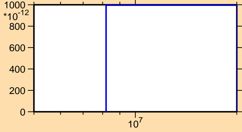
\sigma vs. E for ^{155}\text{Tm}(n,3n\alpha)
