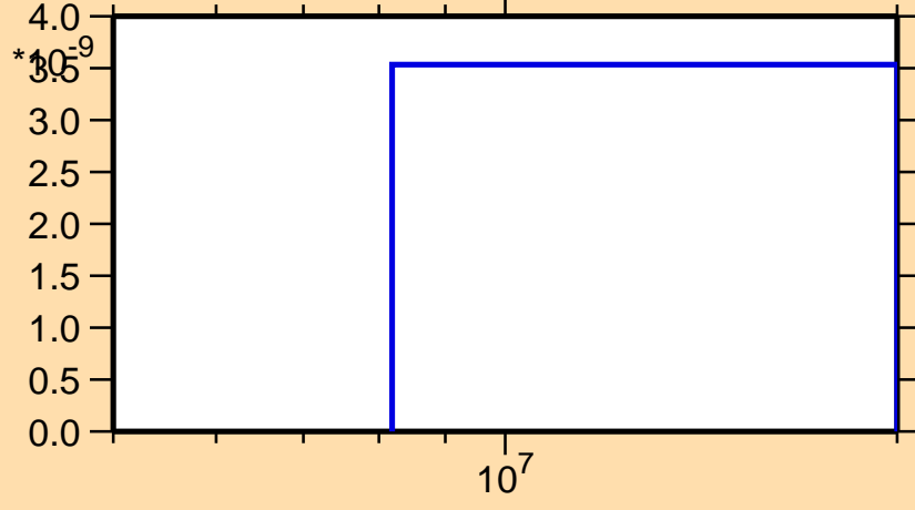
\sigma vs. E for ^{155}\text{Tm}(n,nt)
