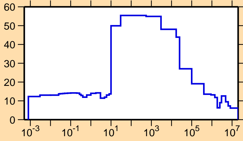
\Delta\sigma/\sigma vs. E for ^{155}\text{Tm}(n,\text{tot.})
