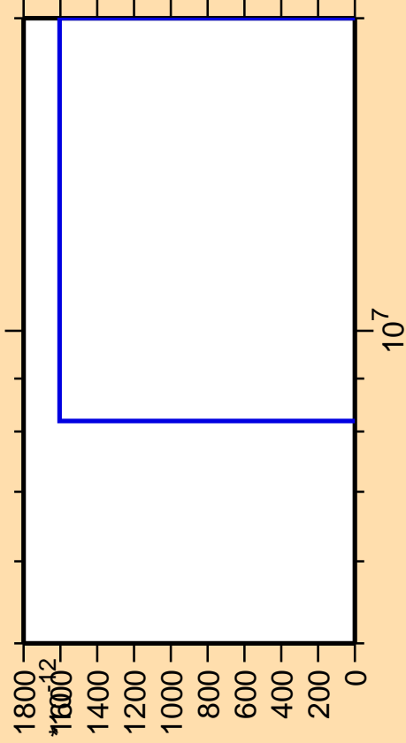
\Delta\sigma/\sigma vs. E for ^{155}\text{Tm} (mt 42)
