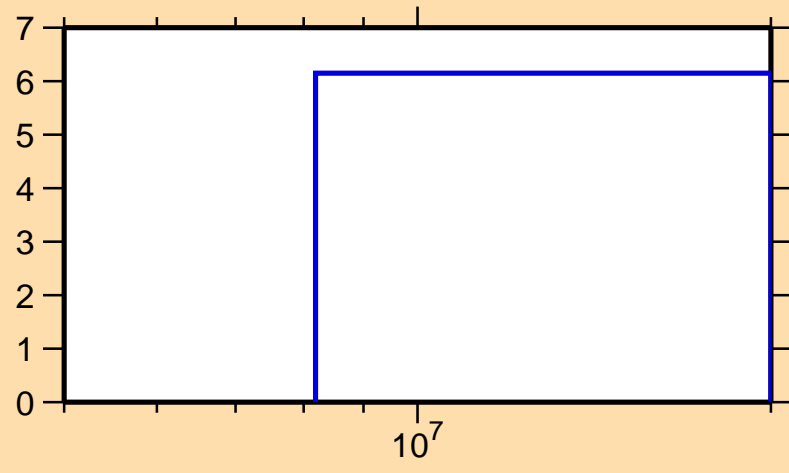
\Delta\sigma/\sigma vs. E for ^{155}\text{Tm}(n,\text{tot.})
