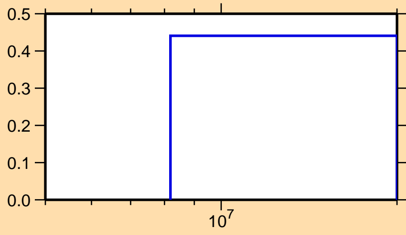
\sigma vs. E for ^{155}\text{Tm}(n,2n)
