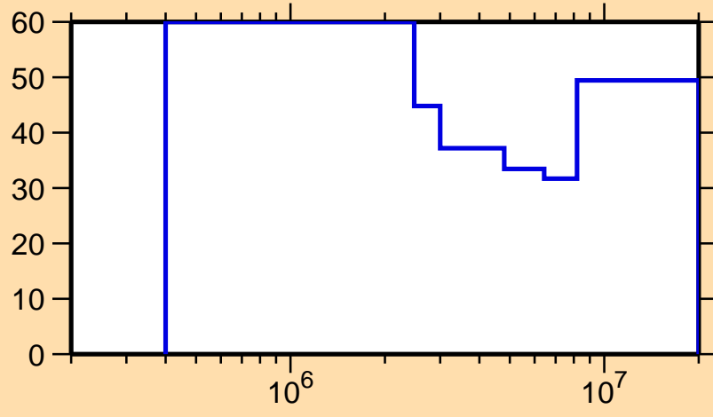
\Delta\sigma/\sigma vs. E for ^{155}\text{Tm}(n,n\text{cont.})
