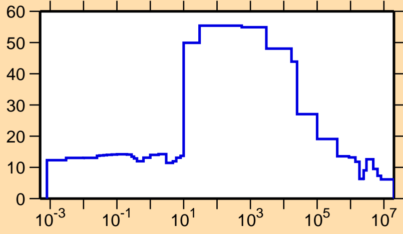
\Delta\sigma/\sigma vs. E for ^{155}\text{Tm}(n,\text{tot.})
