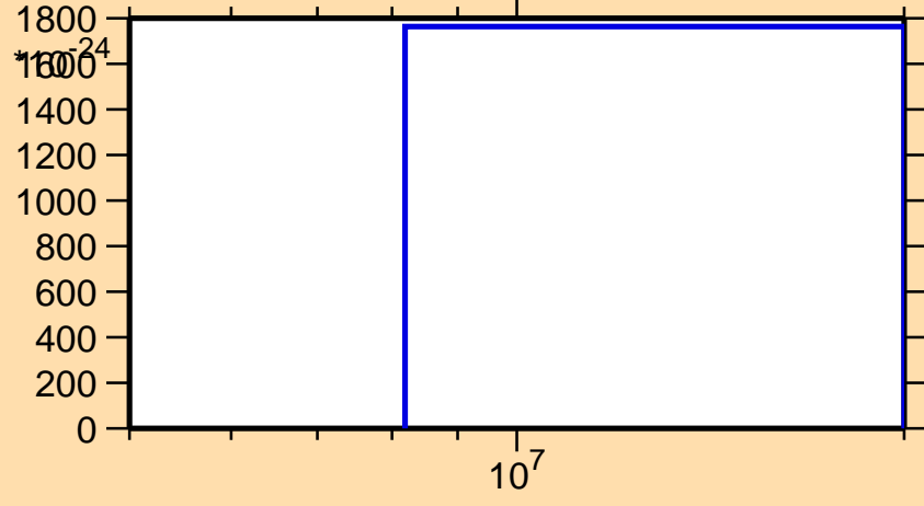
\sigma vs. E for ^{155}\text{Tm} (mt 42)
