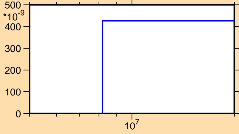
\sigma vs. E for ^{155}\text{Tm}(n,3n)
