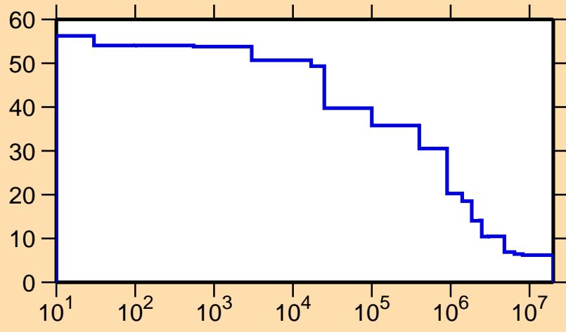
\Delta\sigma/\sigma vs. E for ^{155}\text{Tm}(n,\text{nonel.})
