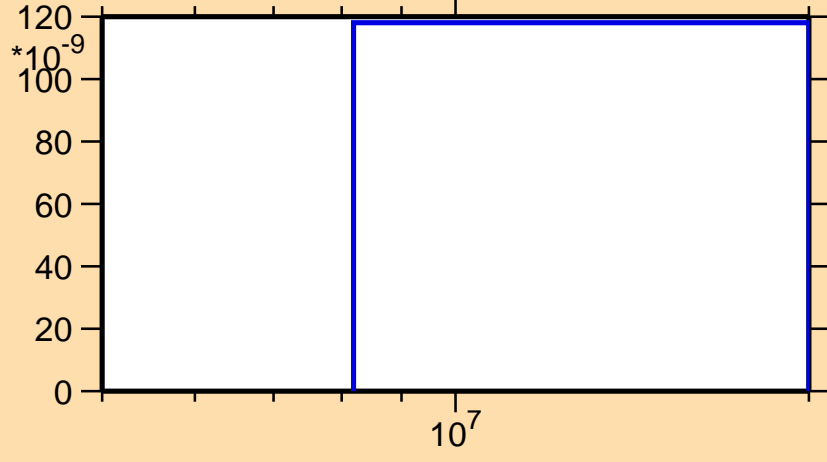
\sigma vs. E for ^{155}\text{Tm}(n,\text{pd})
