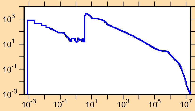
\sigma vs. E for ^{156}\text{Tm}(n,\gamma)
