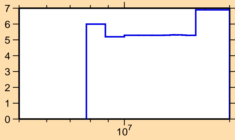
\Delta\sigma/\sigma vs. E for ^{156}\text{Tm}(n,\text{tot.})
