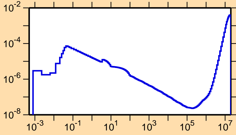
\sigma vs. E for ^{156}\text{Tm}(n,p\alpha)
