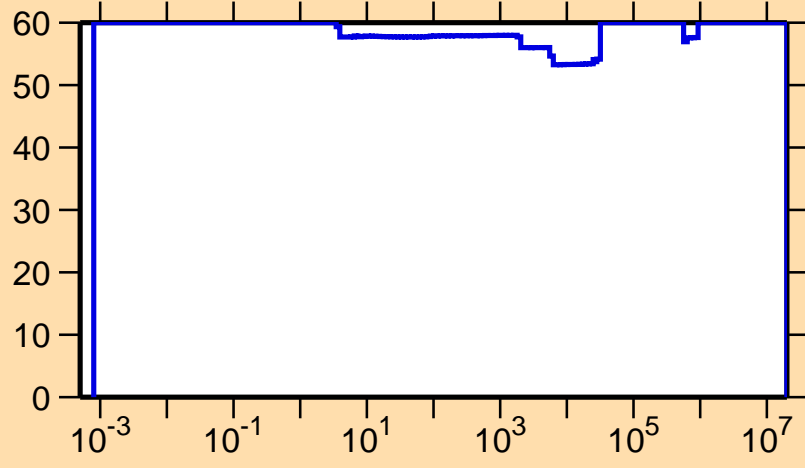
\Delta\sigma/\sigma vs. E for ^{156}\text{Tm}(n,p)
