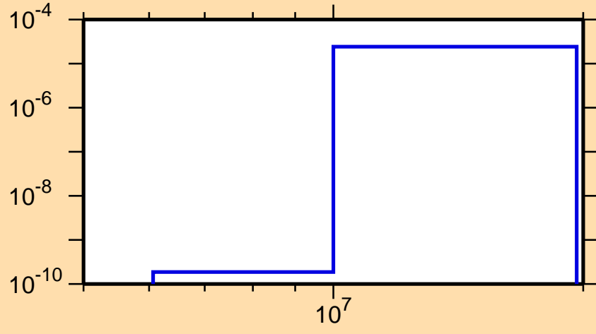
\sigma vs. E for ^{156}\text{Tm} (mt 45)
