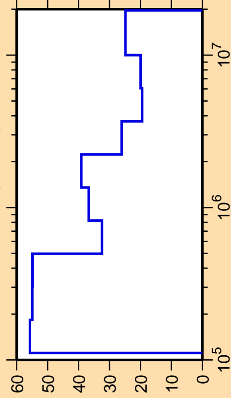
\Delta\sigma/\sigma vs. E for ^{156}\text{Tm}(n,\text{inel.})
