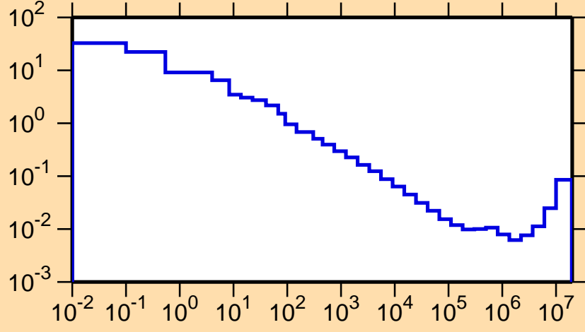
\sigma vs. E for ^{156}\text{Tm}(n,\alpha)
