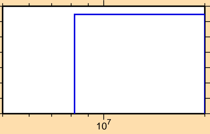
\sigma vs. E for ^{156}\text{Tm}(n,\text{pt})
