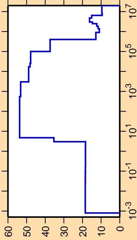
\Delta\sigma/\sigma vs. E for ^{156}\text{Tm}(n,\text{el.})
