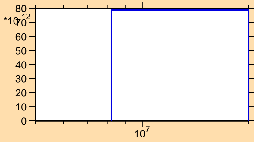
\sigma vs. E for ^{156}\text{Tm} (mt 34)
