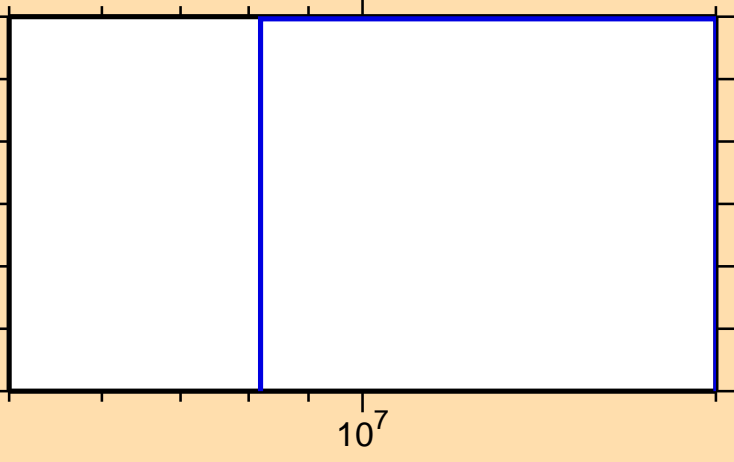
\sigma vs. E for ^{156}\text{Tm}(n,\text{nd})
