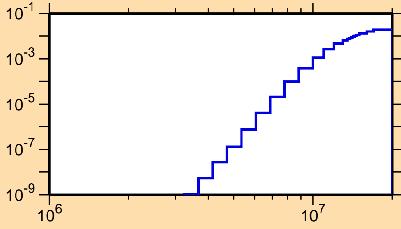
\sigma vs. E for ^{157}\text{Tm}(n,d)
