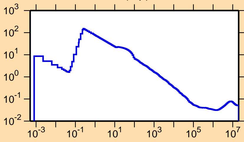
\sigma vs. E for ^{157}\text{Tm}(n,p)
