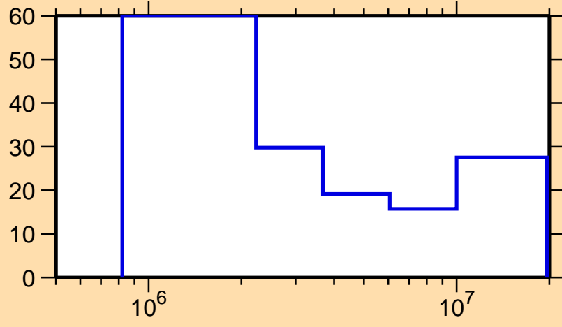
\Delta\sigma/\sigma vs. E for ^{157}\text{Tm}(n,n\text{cont.})
