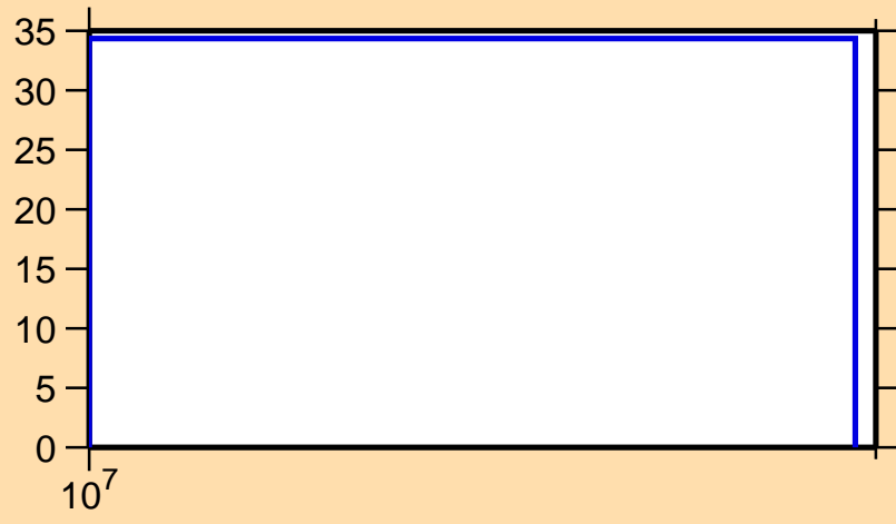
\Delta\sigma/\sigma vs. E for ^{157}\text{Tm}(n,2n)
