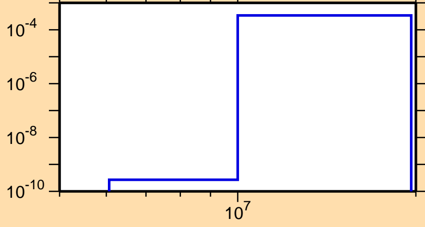
\sigma vs. E for ^{157}\text{Tm}(n,t)
