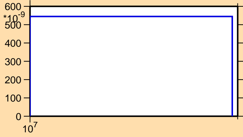
\sigma vs. E for ^{157}\text{Tm}(n,\text{nd})
