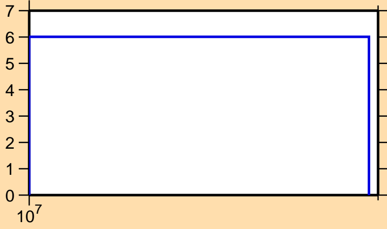
\Delta\sigma/\sigma vs. E for ^{157}\text{Tm}(n,\text{nonel.})
