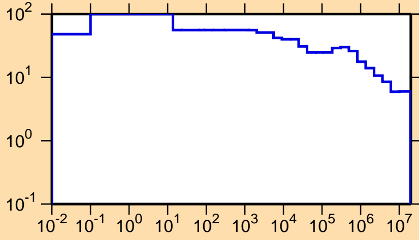
\Delta\sigma/\sigma vs. E for ^{157}\text{Tm}(n,\text{nonel.})
