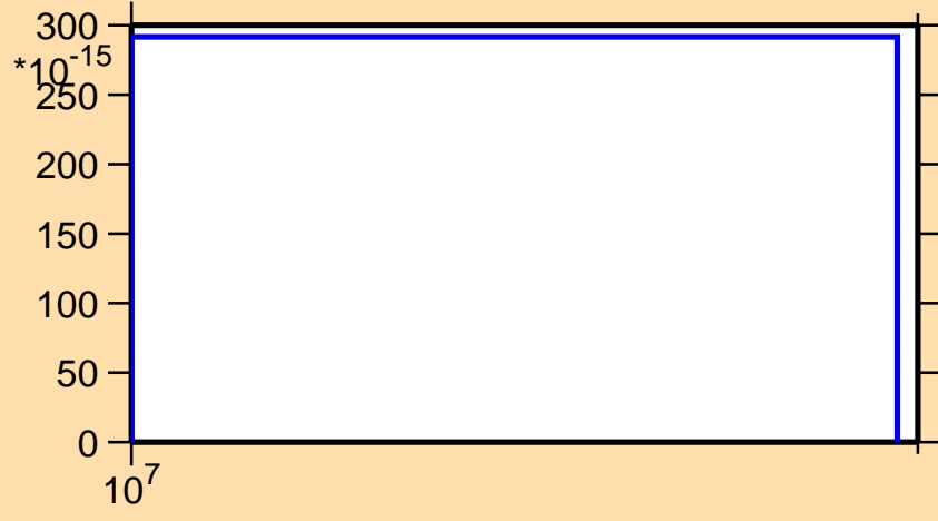
\sigma vs. E for ^{157}\text{Tm} (mt 34)
