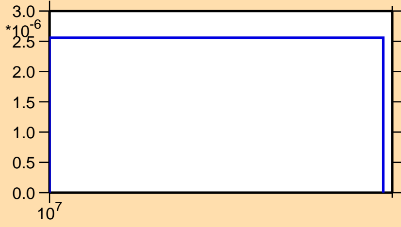
\sigma vs. E for ^{157}\text{Tm}(n,3n)
