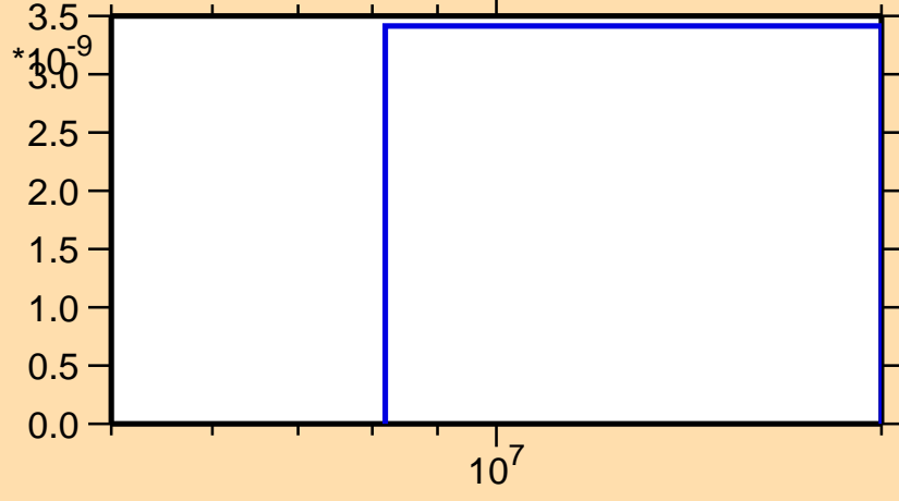
\sigma vs. E for ^{157}\text{Tm}(n,nt)
