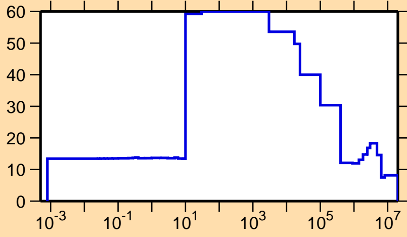
\Delta\sigma/\sigma vs. E for ^{157}\text{Tm}(n,el.)
