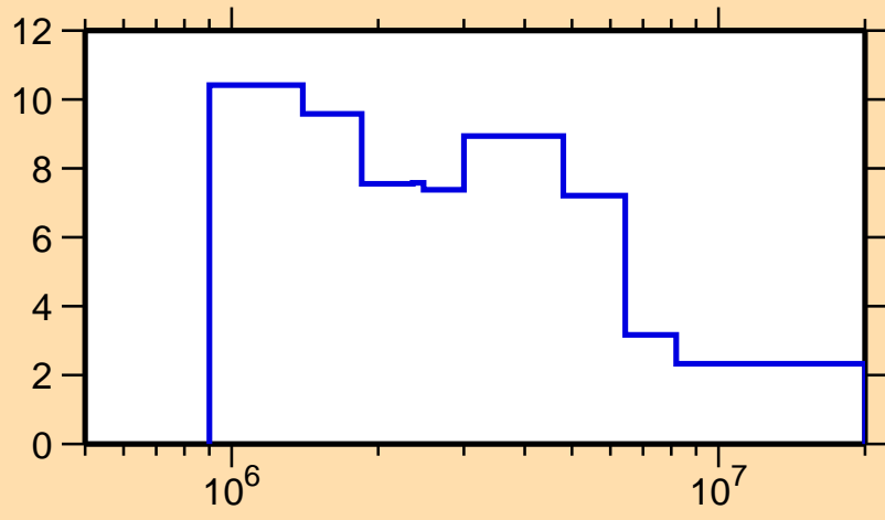
\Delta\sigma/\sigma vs. E for ^{157}\text{Tm}(n, tot.)
