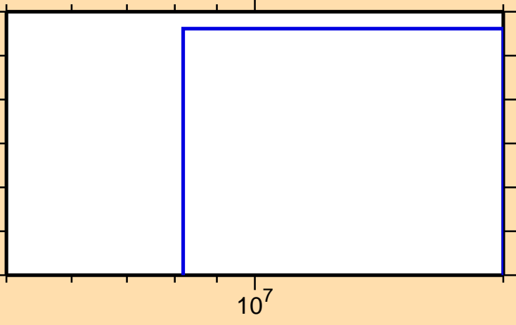
\sigma vs. E for ^{157}\text{Tm}(n,\text{He}3)
