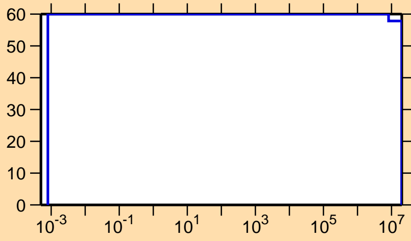
\Delta\sigma/\sigma vs. E for ^{157}\text{Tm}(n,p)
