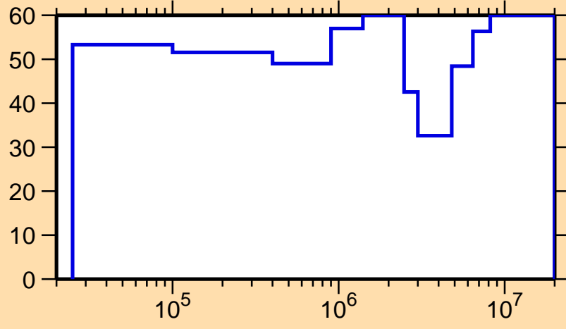
\Delta\sigma/\sigma vs. E for ^{157}\text{Tm}(n,n_1)
