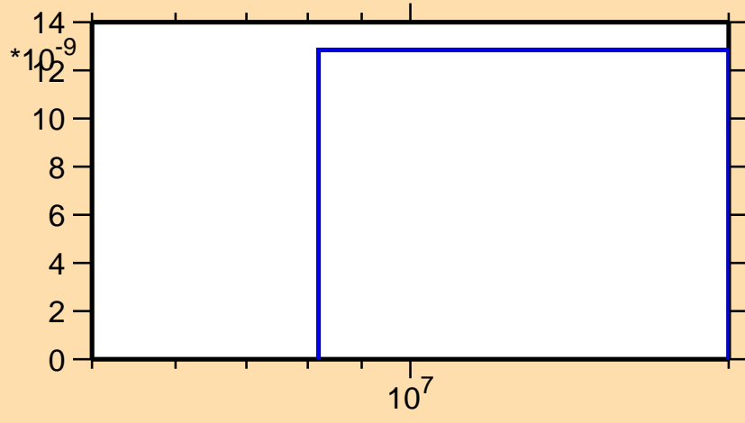
\sigma vs. E for ^{157}\text{Tm}(\text{mt117})
