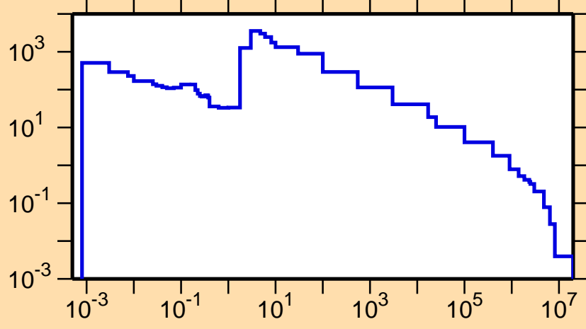
\sigma vs. E for ^{158}\text{Tm}(n,\gamma)
