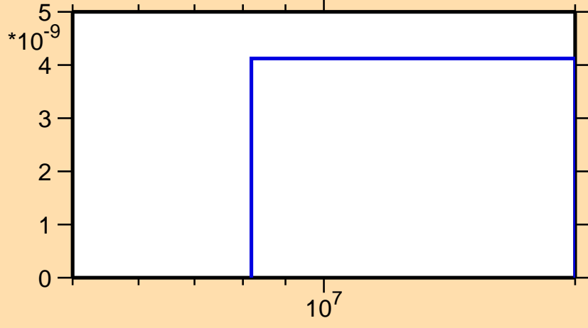
\sigma vs. E for ^{158}\text{Tm}(n,nt)
