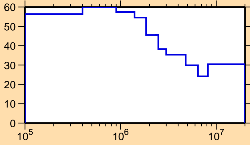
\Delta\sigma/\sigma vs. E for ^{158}\text{Tm}(n,n\text{cont.})
