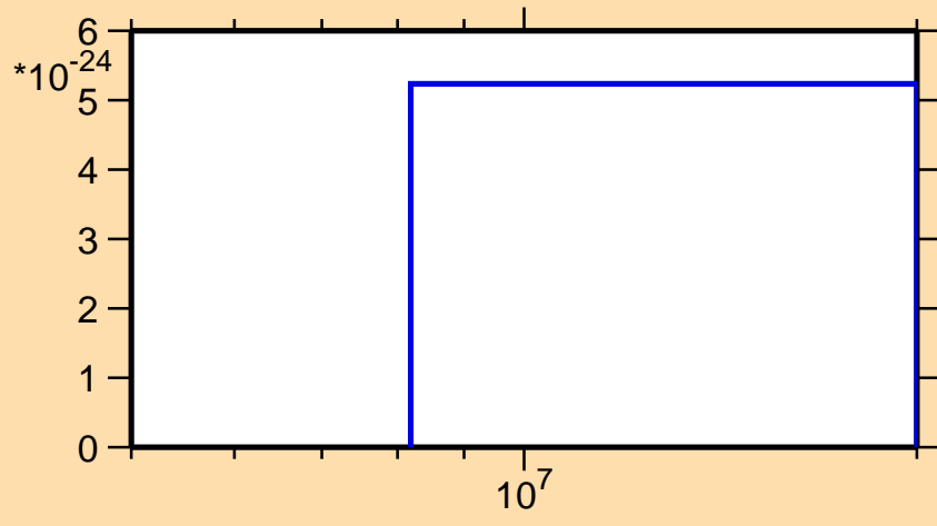
\sigma vs. E for ^{158}\text{Tm} (mt 42)
