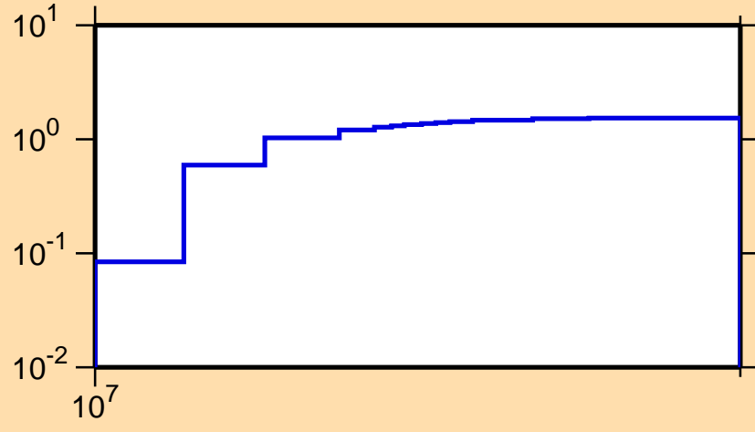
\sigma vs. E for ^{159}\text{Tm}(n,2n)
