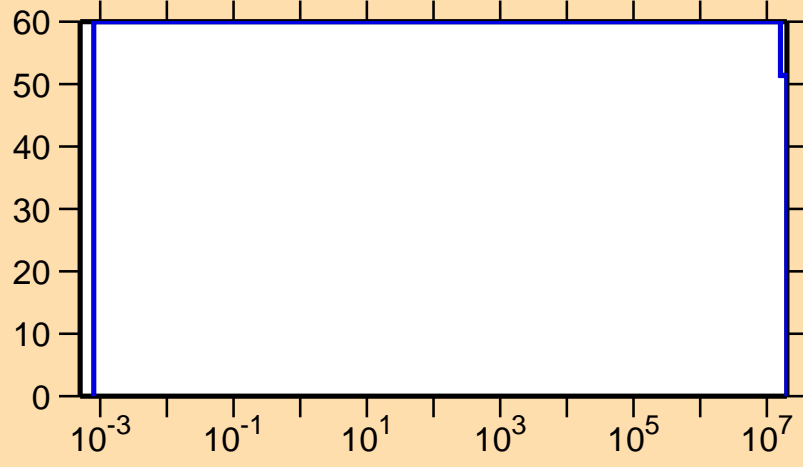
\Delta\sigma/\sigma vs. E for ^{159}\text{Tm}(n,p)
