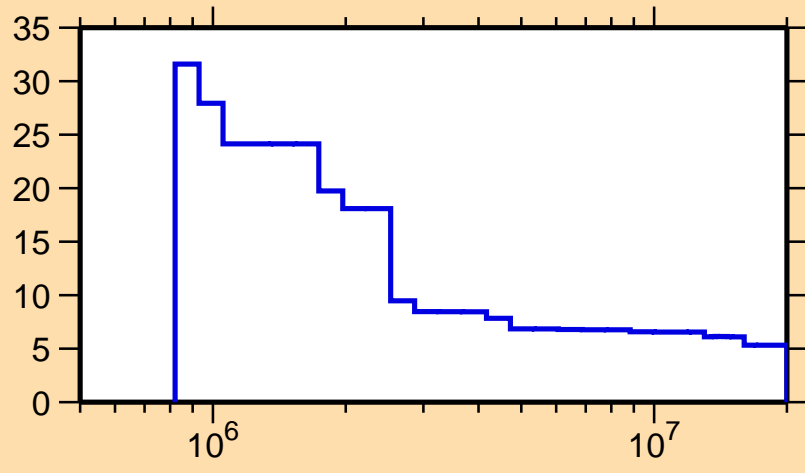
\Delta\sigma/\sigma vs. E for ^{159}\text{Tm}(n, \text{nonel.})
