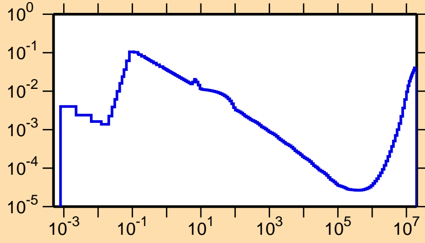
\sigma vs. E for ^{159}\text{Tm}(n,\alpha)
