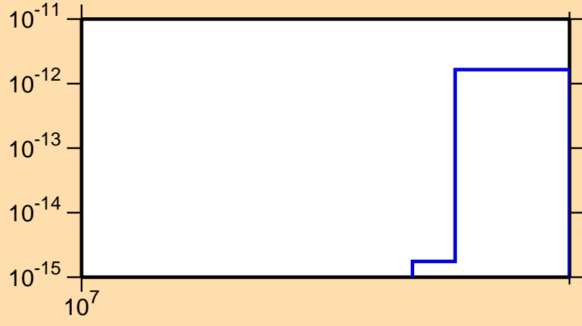
\sigma vs. E for ^{159}\text{Tm} (mt 34)
