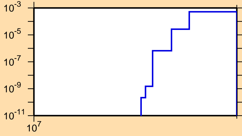
\sigma vs. E for ^{159}\text{Tm}(n,2np)
