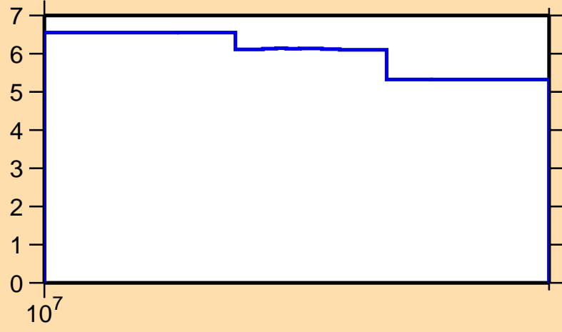
\Delta\sigma/\sigma vs. E for ^{159}\text{Tm}(n,\text{nonel.})
