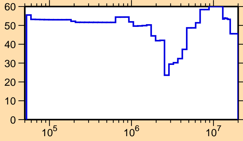
\Delta\sigma/\sigma vs. E for ^{159}\text{Tm}(n,n_1)
