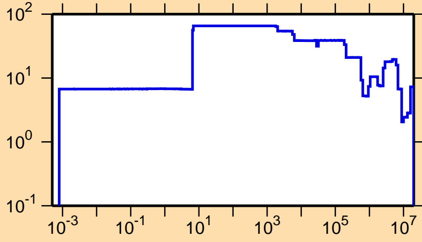
\Delta\sigma/\sigma vs. E for ^{159}\text{Tm}(n,\text{el.})
