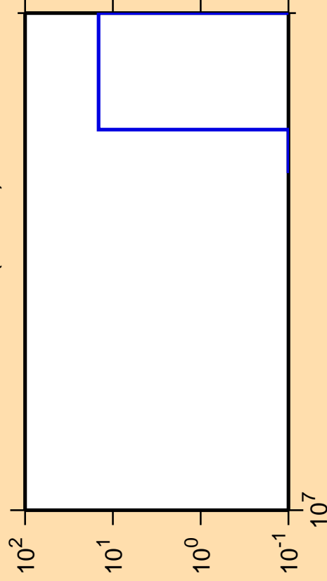
\Delta\sigma/\sigma vs. E for ^{159}\text{Tm} (mt 34)
