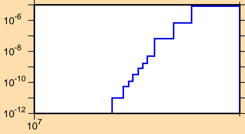
\sigma vs. E for ^{159}\text{Tm}(n,2n\alpha)
