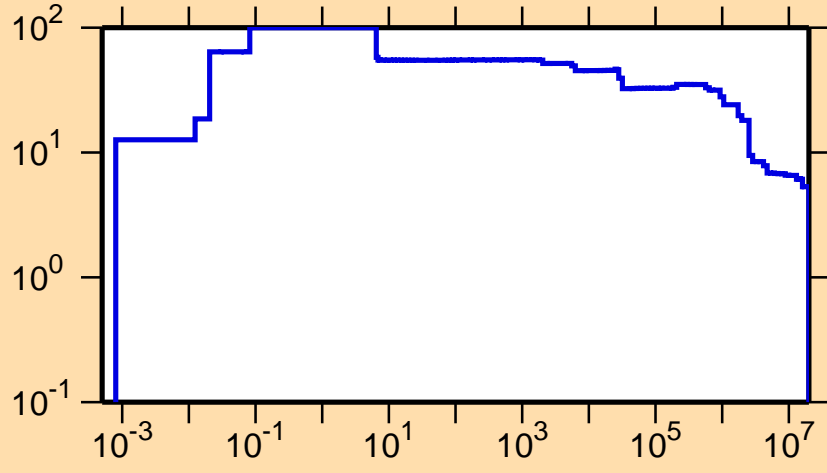
\Delta\sigma/\sigma vs. E for ^{159}\text{Tm}(n,\text{nonel.})
