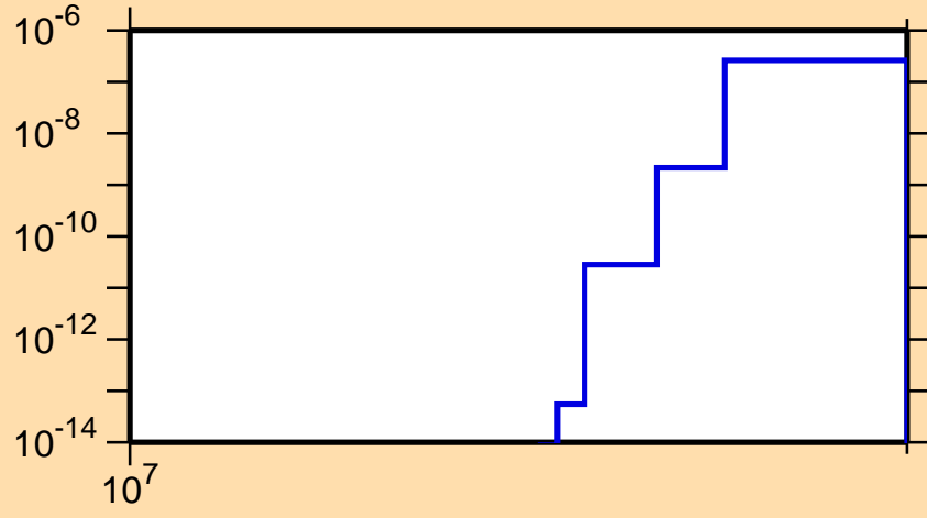
\sigma vs. E for ^{159}\text{Tm}(n,nt)
