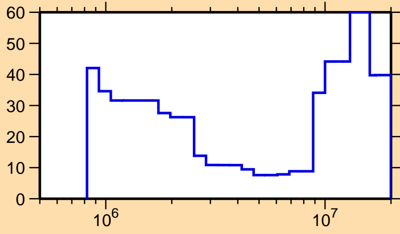
\Delta\sigma/\sigma vs. E for ^{159}\text{Tm}(n,\text{inel.})
