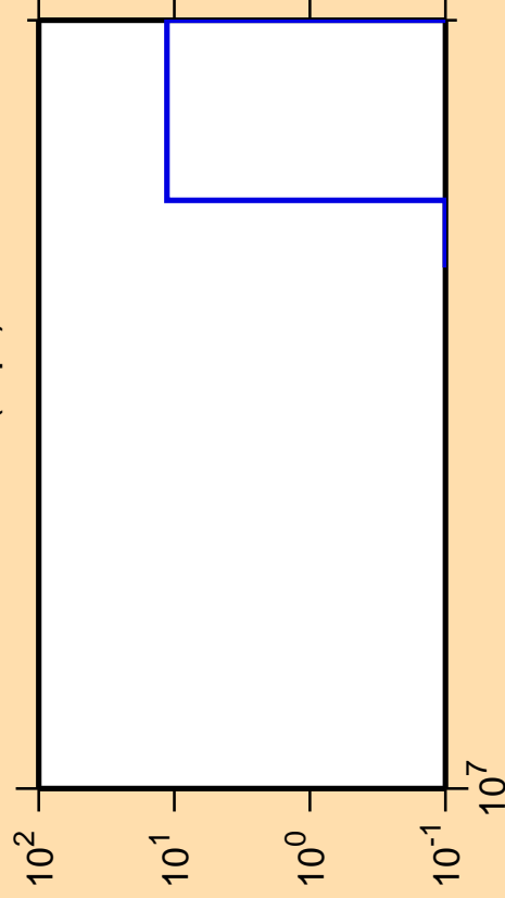
\Delta\sigma/\sigma vs. E for ^{159}\text{Tm}(n,\text{pt})
