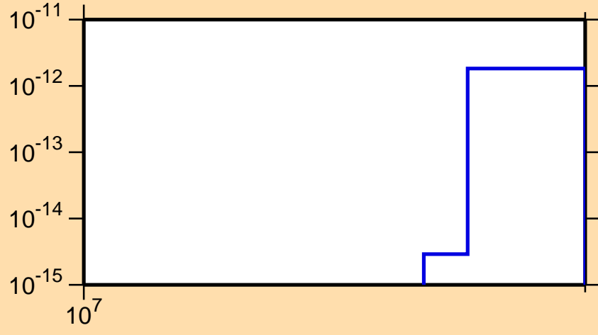
\sigma vs. E for ^{159}\text{Tm}(n,\text{pt})
