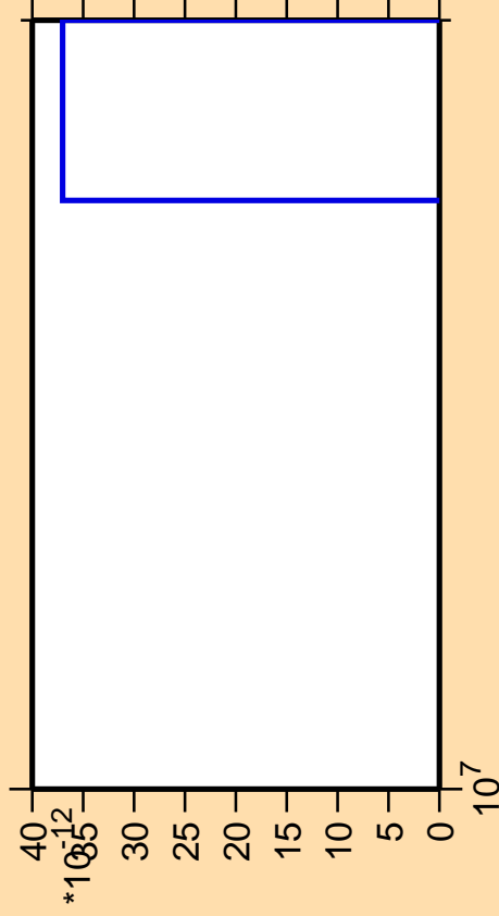
\Delta\sigma/\sigma vs. E for ^{159}\text{Tm} (mt 42)
