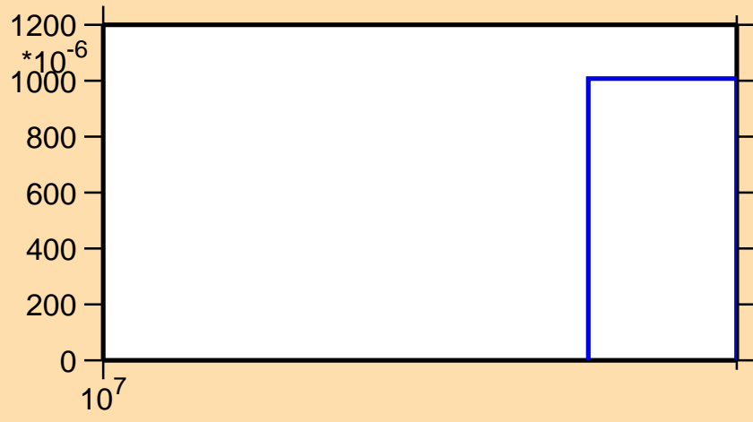
\sigma vs. E for ^{159}\text{Tm}(n,3n)
