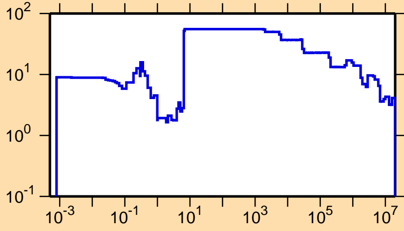
\Delta\sigma/\sigma vs. E for ^{159}\text{Tm}(n,\text{tot.})
