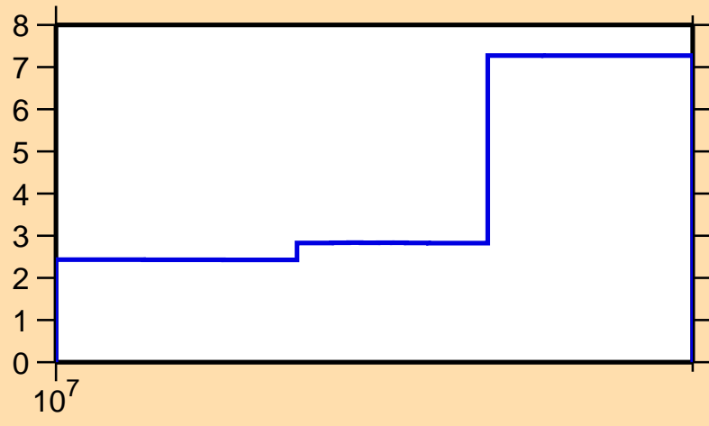
\Delta\sigma/\sigma vs. E for ^{159}\text{Tm}(n,\text{el.})
