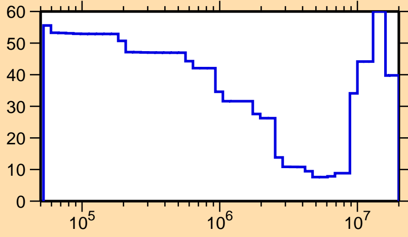
\Delta\sigma/\sigma vs. E for ^{159}\text{Tm}(n,\text{inel.})
