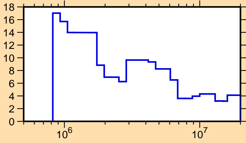
\Delta\sigma/\sigma vs. E for ^{159}\text{Tm}(n, \text{tot.})
