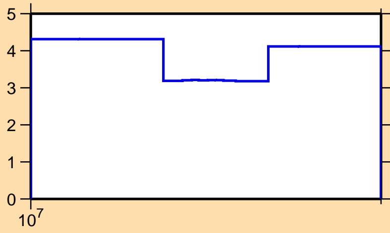
\Delta\sigma/\sigma vs. E for ^{159}\text{Tm}(n,\text{tot.})
