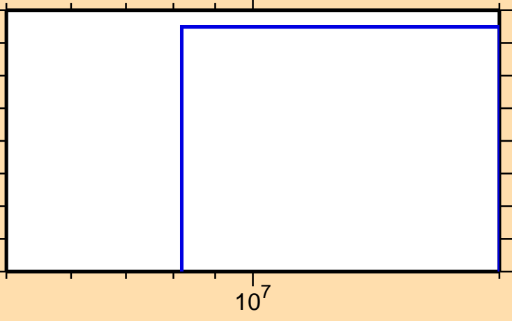
\sigma vs. E for ^{159}\text{Tm}(n,\text{pt})
