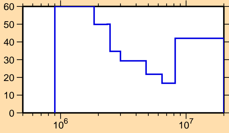
\Delta\sigma/\sigma vs. E for ^{159}\text{Tm}(n,n\text{cont.})
