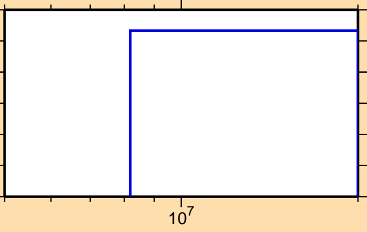
\sigma vs. E for ^{159}\text{Tm}(n,2np)
