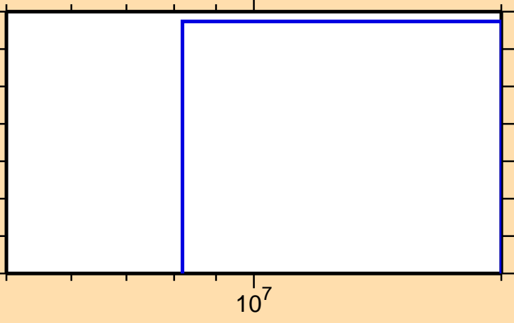
\sigma vs. E for ^{159}\text{Tm} (mt 34)
