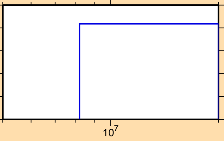
\sigma vs. E for ^{159}\text{Tm}(n,\text{He}3)
