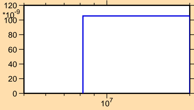
\sigma vs. E for ^{159}\text{Tm}(n,\text{nd})
