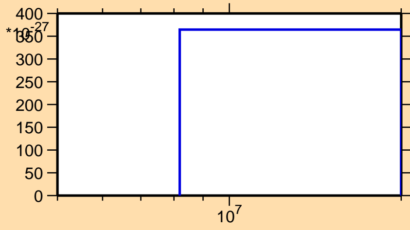
\sigma vs. E for ^{159}\text{Tm} (mt 42)
