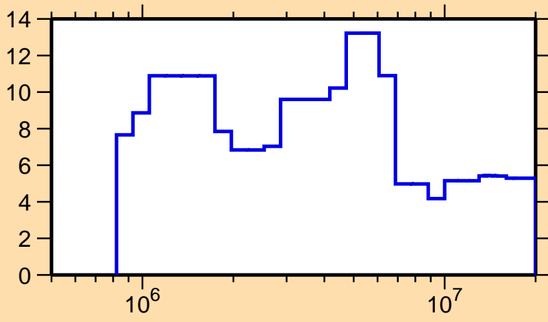
\Delta\sigma/\sigma vs. E for ^{160}\text{Tm}(n, el.)
