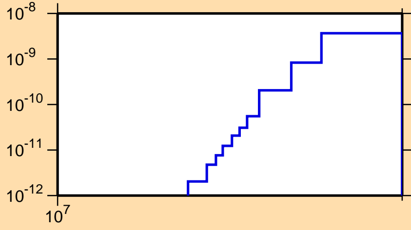
\sigma vs. E for ^{160}\text{Tm}(\text{mt117})
