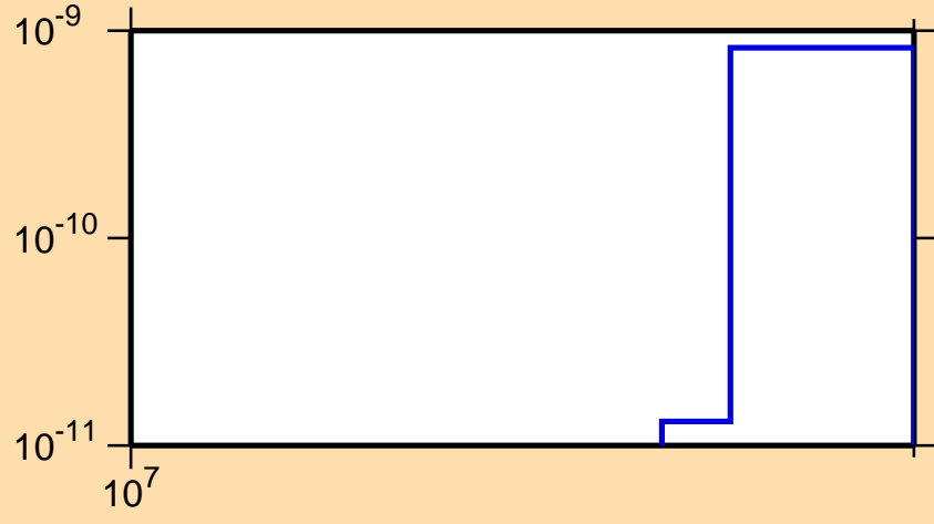
\sigma vs. E for ^{160}\text{Tm}(n,pt)
