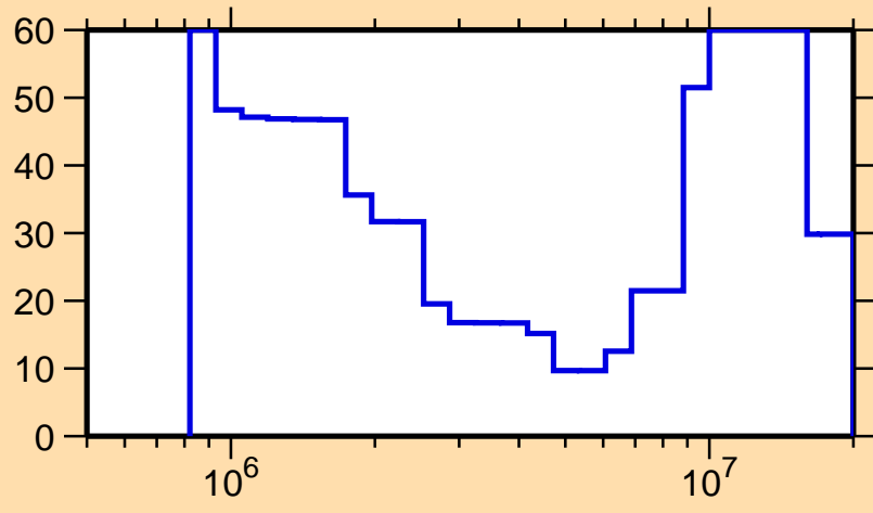
\Delta\sigma/\sigma vs. E for ^{160}\text{Tm}(n,n\text{cont.})
