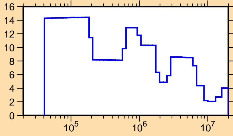
\Delta\sigma/\sigma vs. E for ^{160}\text{Tm}(n,\text{tot.})
