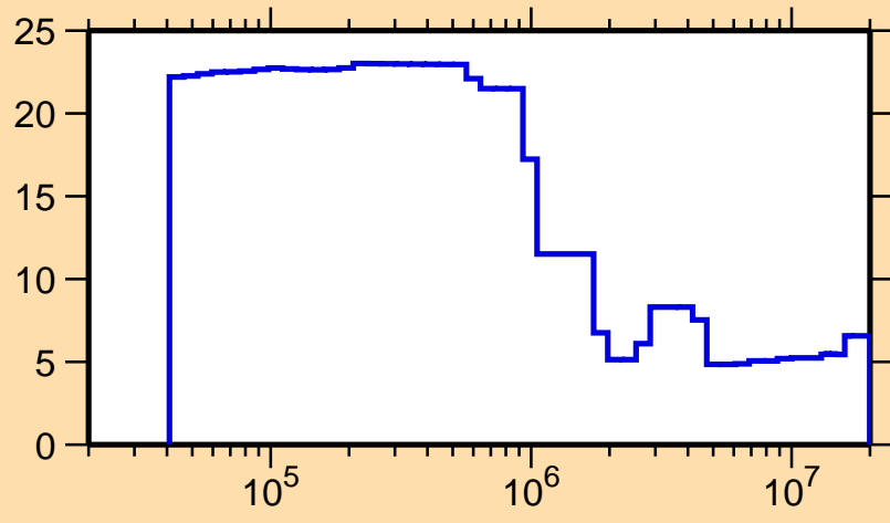
\Delta\sigma/\sigma vs. E for ^{160}\text{Tm}(n,\text{nonel.})
