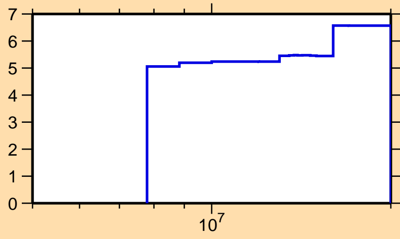
\Delta\sigma/\sigma vs. E for ^{160}\text{Tm}(n,\text{nonel.})
