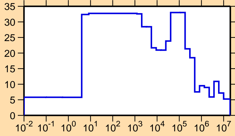
\Delta\sigma/\sigma vs. E for ^{160}\text{Tm}(n,el.)
