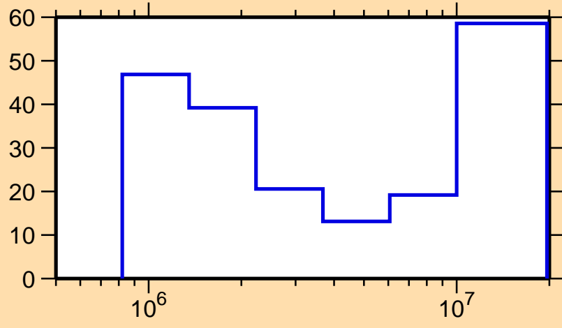
\Delta\sigma/\sigma vs. E for ^{160}\text{Tm}(n,ncont.)
