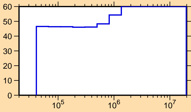
\Delta\sigma/\sigma vs. E for ^{160}\text{Tm}(n,n_1)
