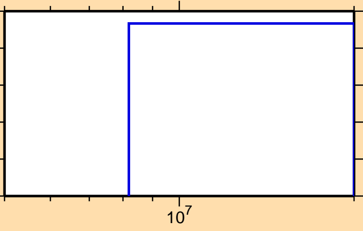
\sigma vs. E for ^{160}\text{Tm} (mt 45)
