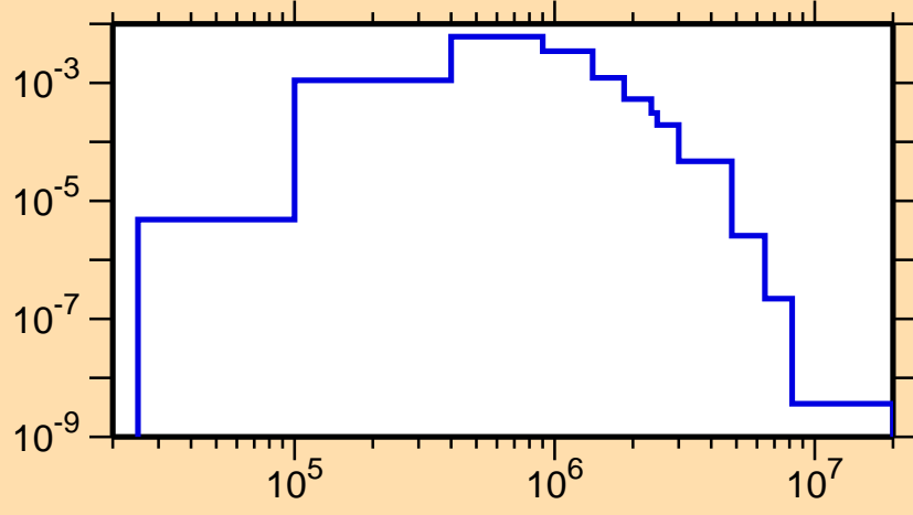
\sigma vs. E for ^{160}\text{Tm}(n,n_3)
