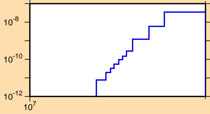
\sigma vs. E for ^{161}\text{Tm} (mt 45)
