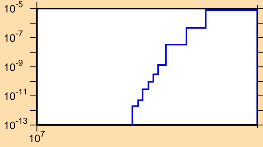
\sigma vs. E for ^{161}\text{Tm}(n,nd)
