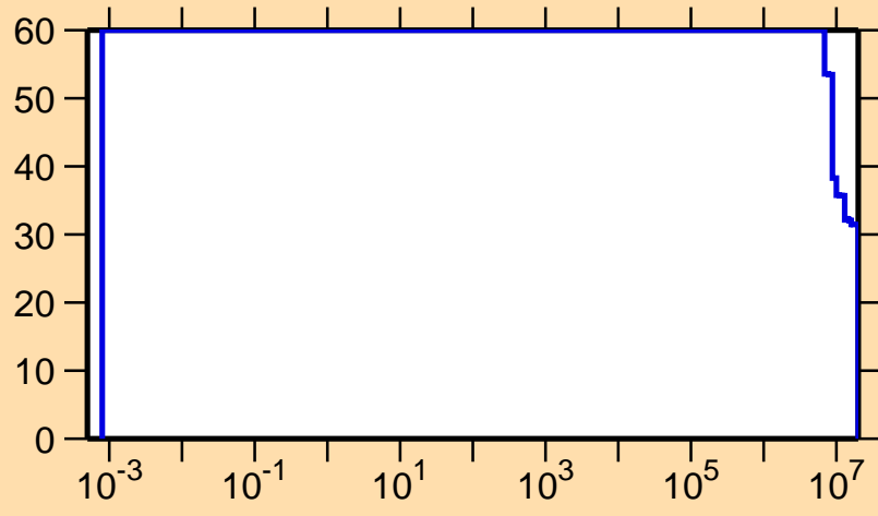
\Delta\sigma/\sigma vs. E for ^{161}\text{Tm}(n,p)
