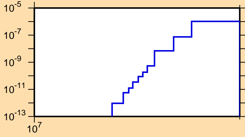
\sigma vs. E for ^{161}\text{Tm}(n,2n\alpha)
