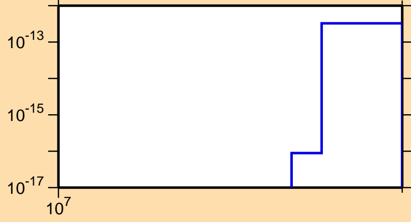
\sigma vs. E for ^{161}\text{Tm} (mt 34)
