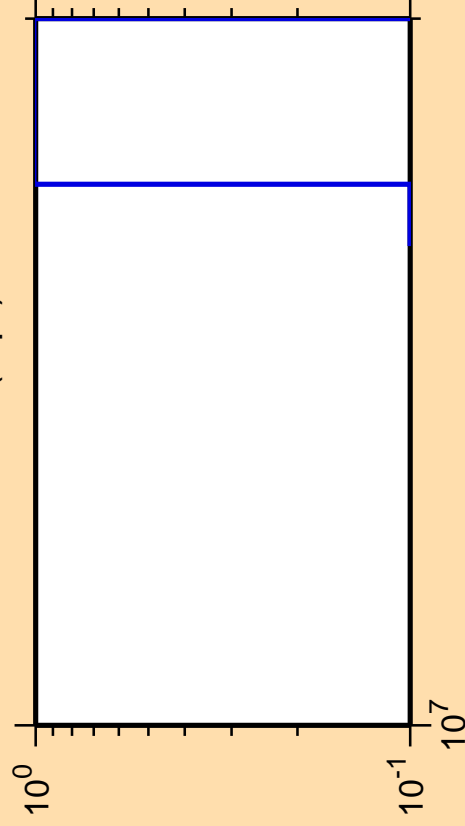
\Delta\sigma/\sigma vs. E for ^{161}\text{Tm}(n,\text{pt})
