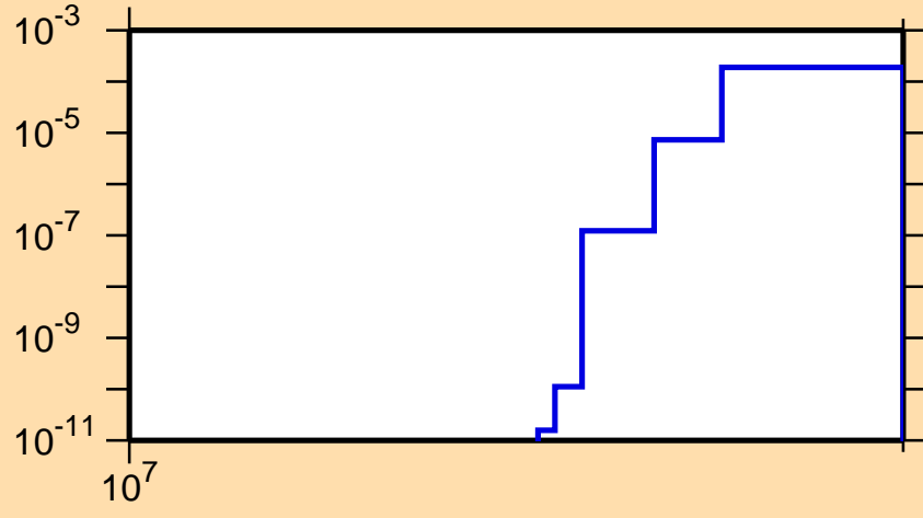
\sigma vs. E for ^{161}\text{Tm}(n,2np)
