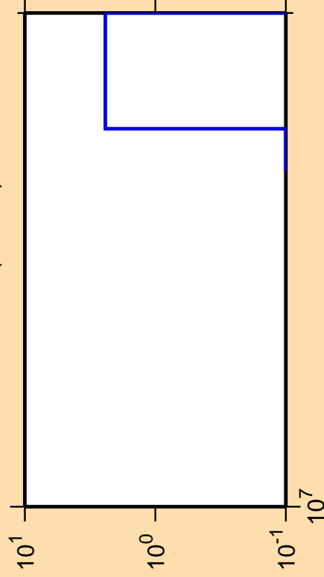
\Delta\sigma/\sigma vs. E for ^{161}\text{Tm} (mt 34)
