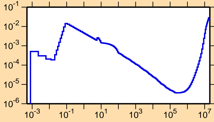
\sigma vs. E for ^{161}\text{Tm}(n,\alpha)
