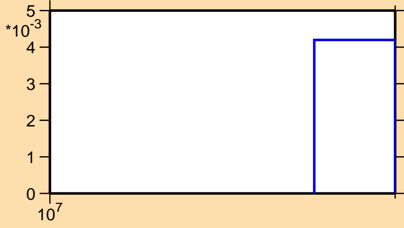
\sigma vs. E for ^{161}\text{Tm}(n,3n)
