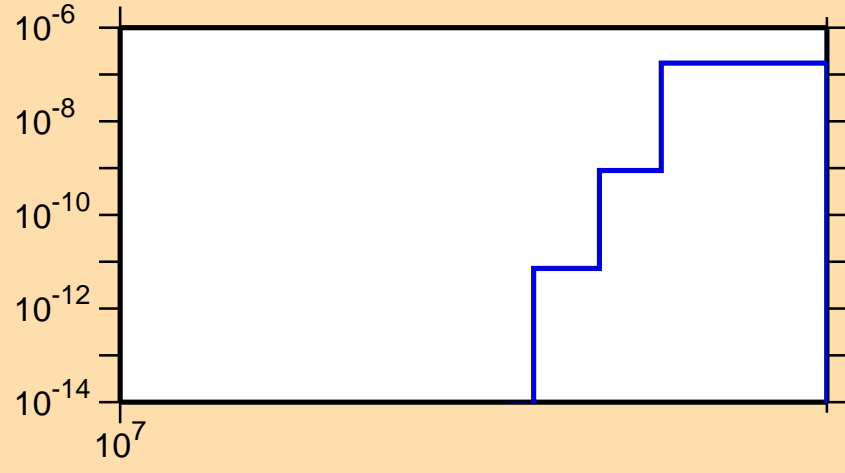
\sigma vs. E for ^{161}\text{Tm}(n,nt)
