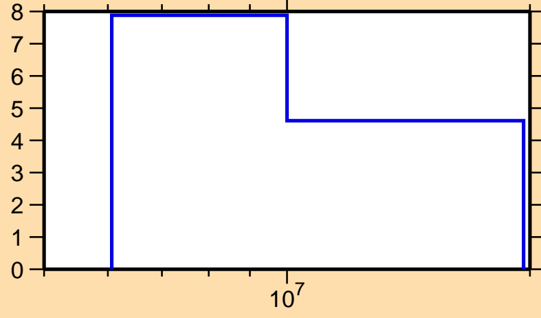
\Delta\sigma/\sigma vs. E for ^{161}\text{Tm}(n,\text{el.})
