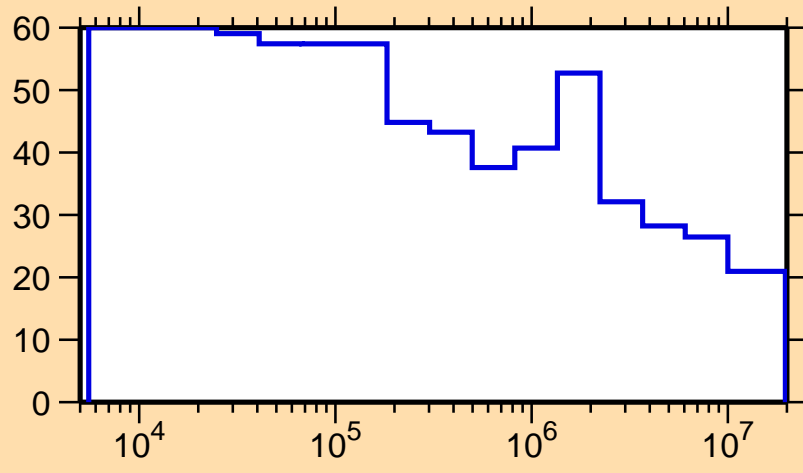
\Delta\sigma/\sigma vs. E for ^{161}\text{Tm}(n,n_1)
