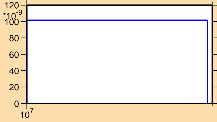
\sigma vs. E for ^{161}\text{Tm}(n,\text{nd})
