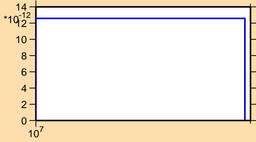
\sigma vs. E for ^{161}\text{Tm}(n,\text{pd})
