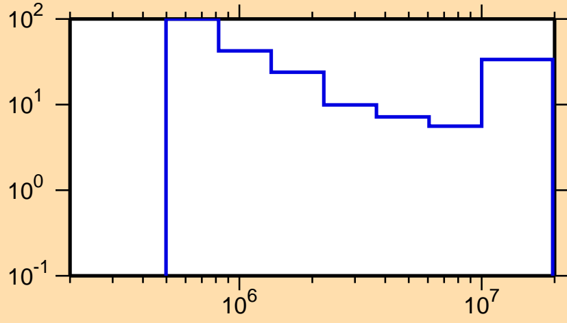
\Delta\sigma/\sigma vs. E for ^{161}\text{Tm}(n,n\text{cont.})
