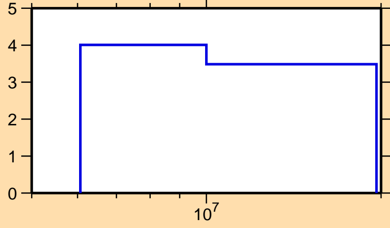
\Delta\sigma/\sigma vs. E for ^{161}\text{Tm}(n,\text{nonel.})
