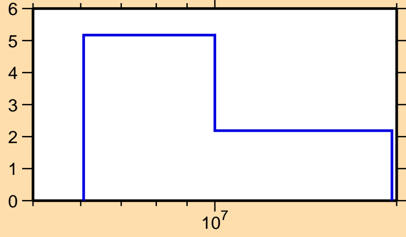
\Delta\sigma/\sigma vs. E for ^{161}\text{Tm}(n,\text{tot.})
