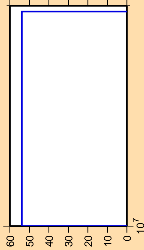
\Delta\sigma/\sigma vs. E for ^{161}\text{Tm}(n,\text{pd})
